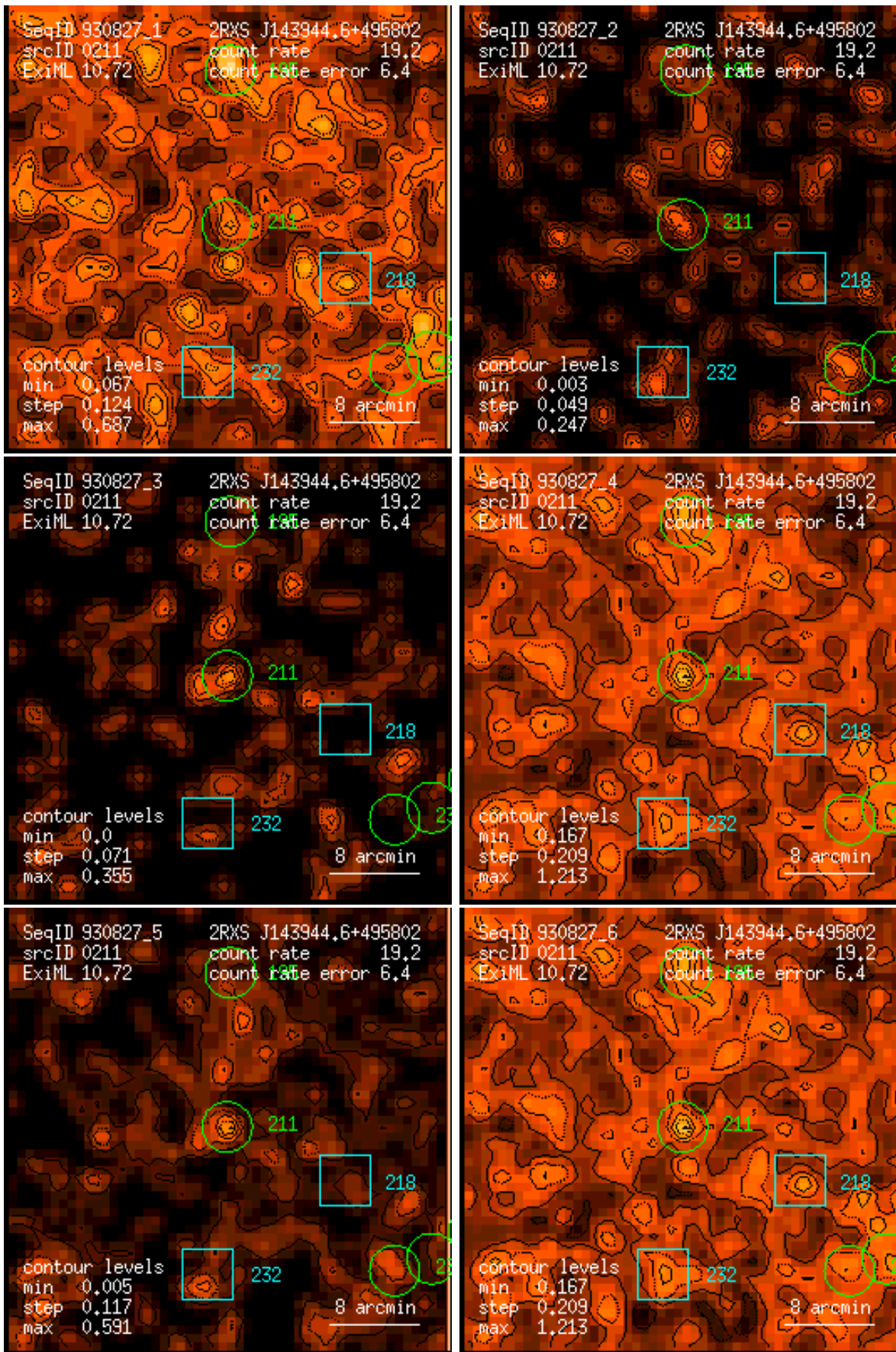
Figure 211: RASS 930827: detection 0211: band rate images, Gaussian filter: (1) PSPC channels 11 – 41, (2) 52 – 90, (3) 91 – 201, (4) 11 – 235, (5) 52 – 201, (6) 11 – 201. Broad band rates in counts/ks. Band rate contour levels in counts/ks/arcmin 2 .
