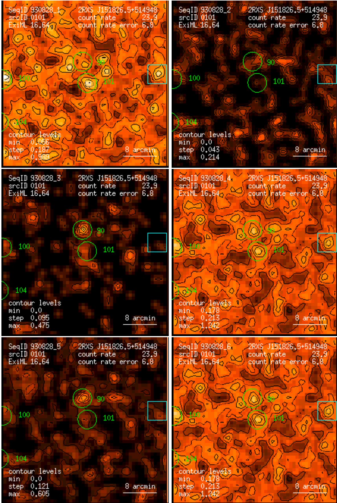
Figure 101: RASS 930828: detection 0101: band rate images, Gaussian filter: (1) PSPC channels 11 – 41, (2) 52 – 90, (3) 91 – 201, (4) 11 – 235, (5) 52 – 201, (6) 11 – 201. Broad band rates in counts/ks. Band rate contour levels in counts/ks/arcmin 2 .
