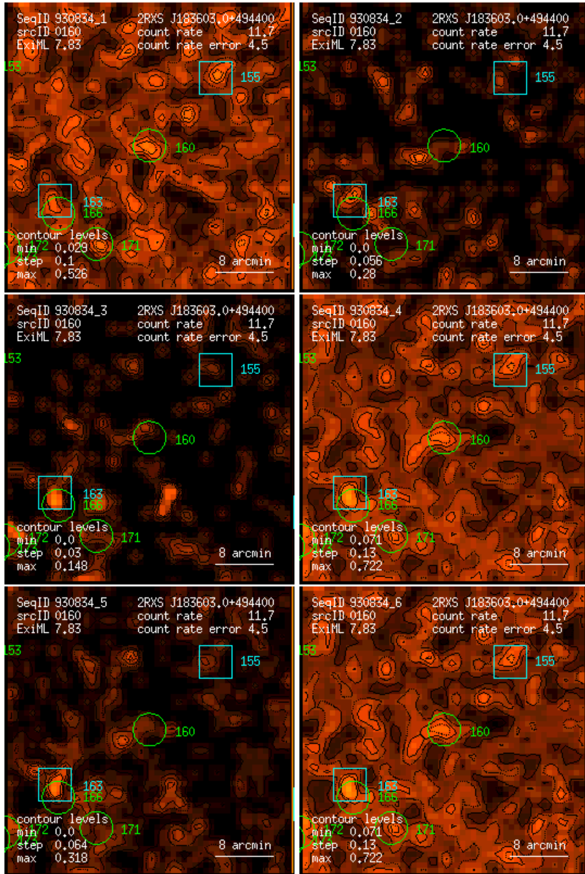
Figure 160: RASS 930834: detection 0160: band rate images, Gaussian filter: (1) PSPC channels 11 – 41, (2) 52 – 90, (3) 91 – 201, (4) 11 – 235, (5) 52 – 201, (6) 11 – 201. Broad band rates in counts/ks. Band rate contour levels in counts/ks/arcmin 2 .
