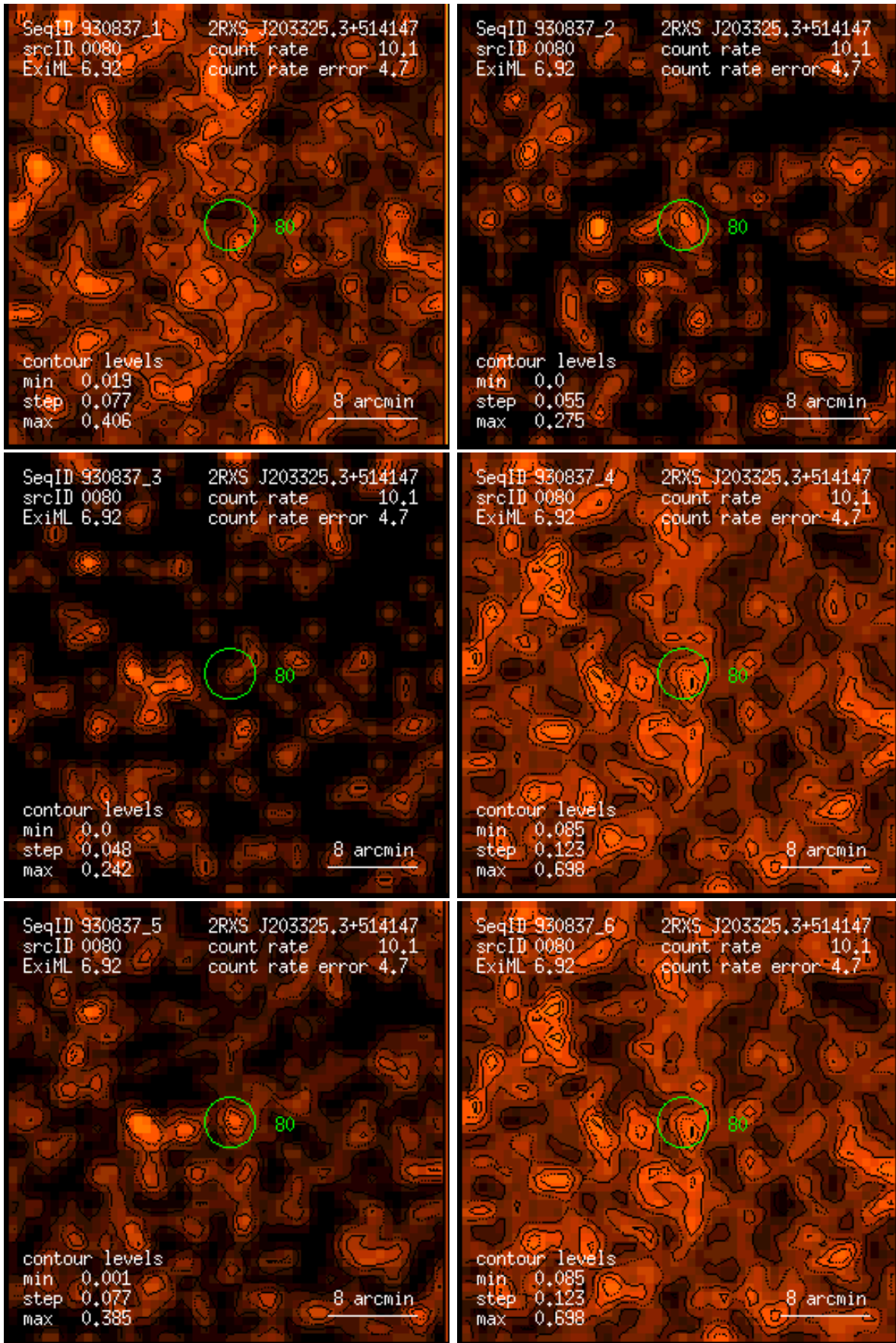
Figure 80: RASS 930837: detection 0080: band rate images, Gaussian filter: (1) PSPC channels 11 – 41, (2) 52 – 90, (3) 91 – 201, (4) 11 – 235, (5) 52 – 201, (6) 11 – 201. Broad band rates in counts/ks. Band rate contour levels in counts/ks/arcmin 2 .
