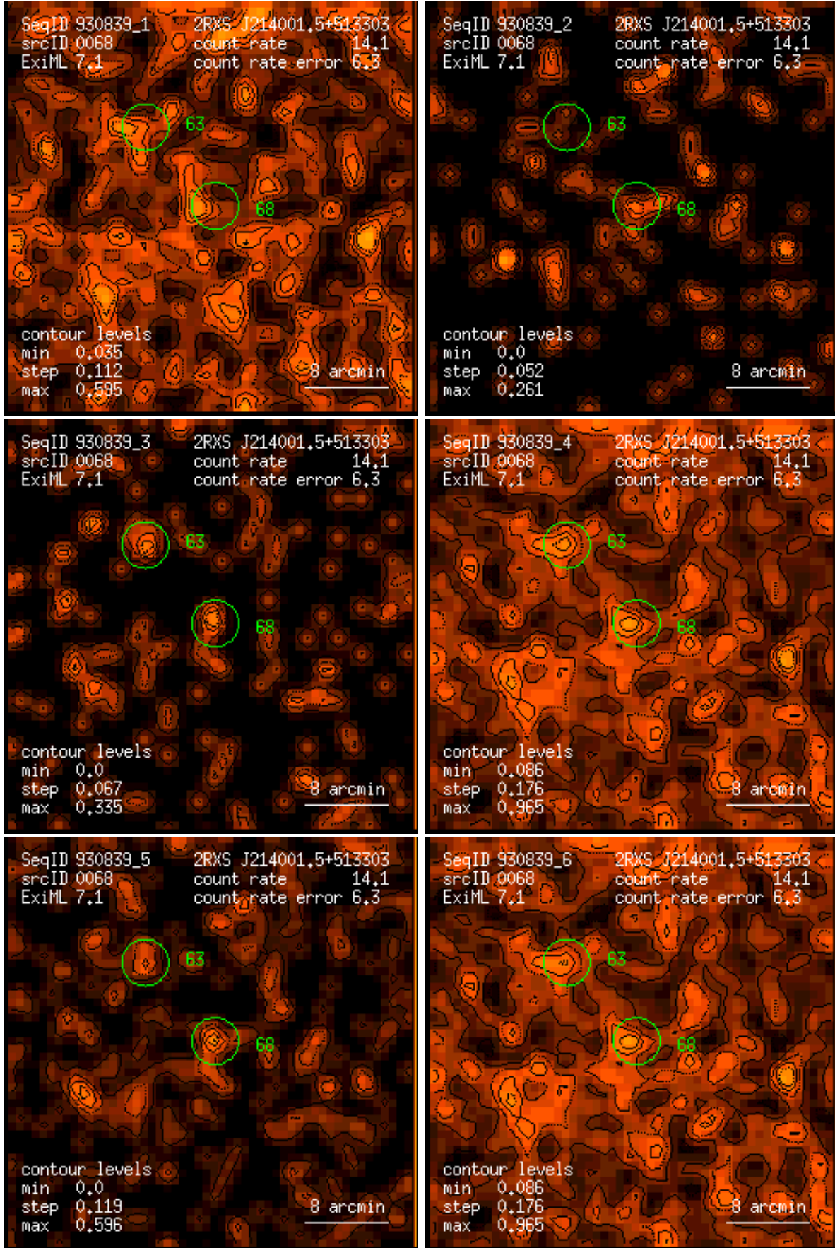
Figure 68: RASS 930839: detection 0068: band rate images, Gaussian filter: (1) PSPC channels 11 – 41, (2) 52 – 90, (3) 91 – 201, (4) 11 – 235, (5) 52 – 201, (6) 11 – 201. Broad band rates in counts/ks. Band rate contour levels in counts/ks/arcmin 2 .
