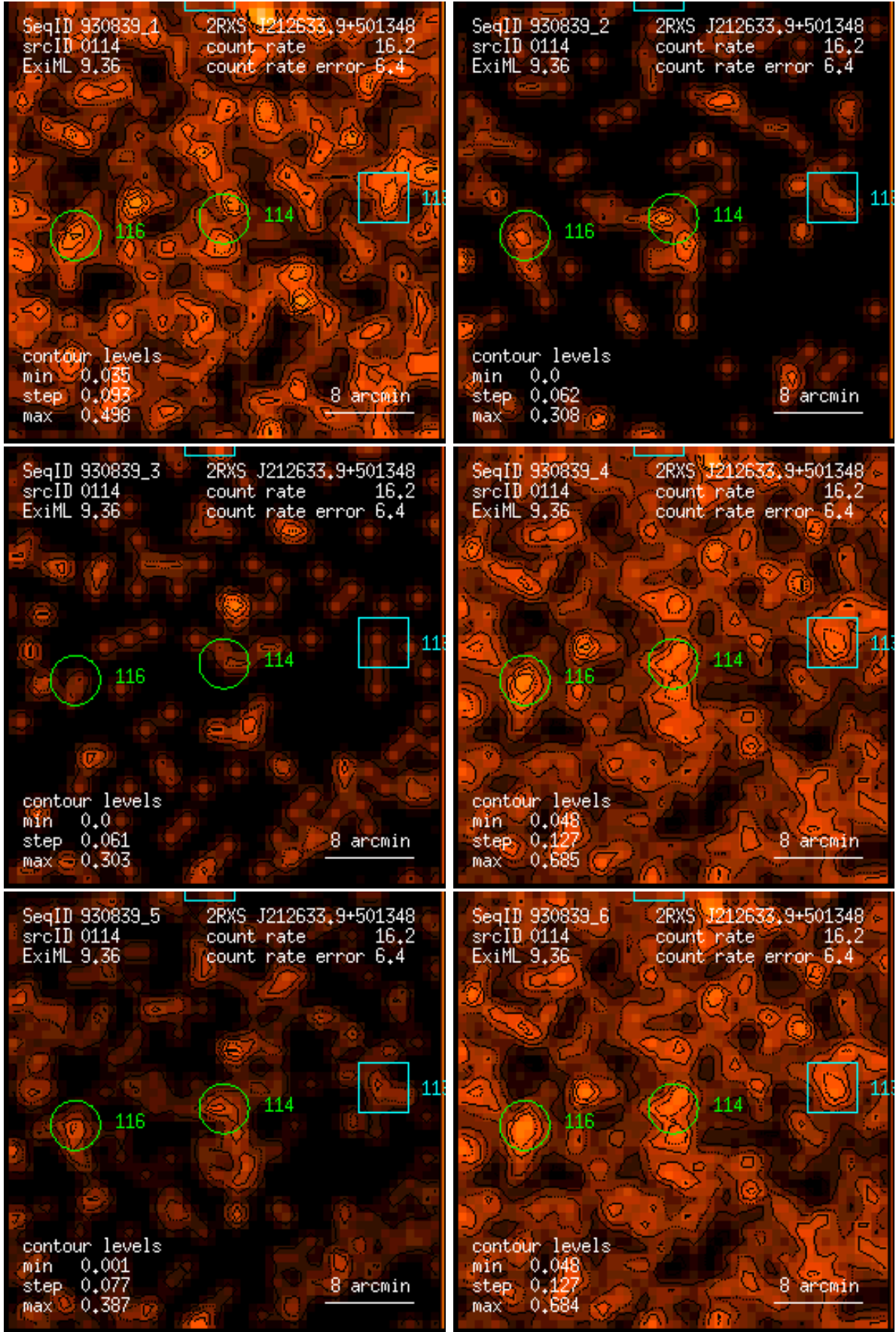
Figure 114: RASS 930839: detection 0114: band rate images, Gaussian filter: (1) PSPC channels 11 – 41, (2) 52 – 90, (3) 91 – 201, (4) 11 – 235, (5) 52 – 201, (6) 11 – 201. Broad band rates in counts/ks. Band rate contour levels in counts/ks/arcmin 2 .
