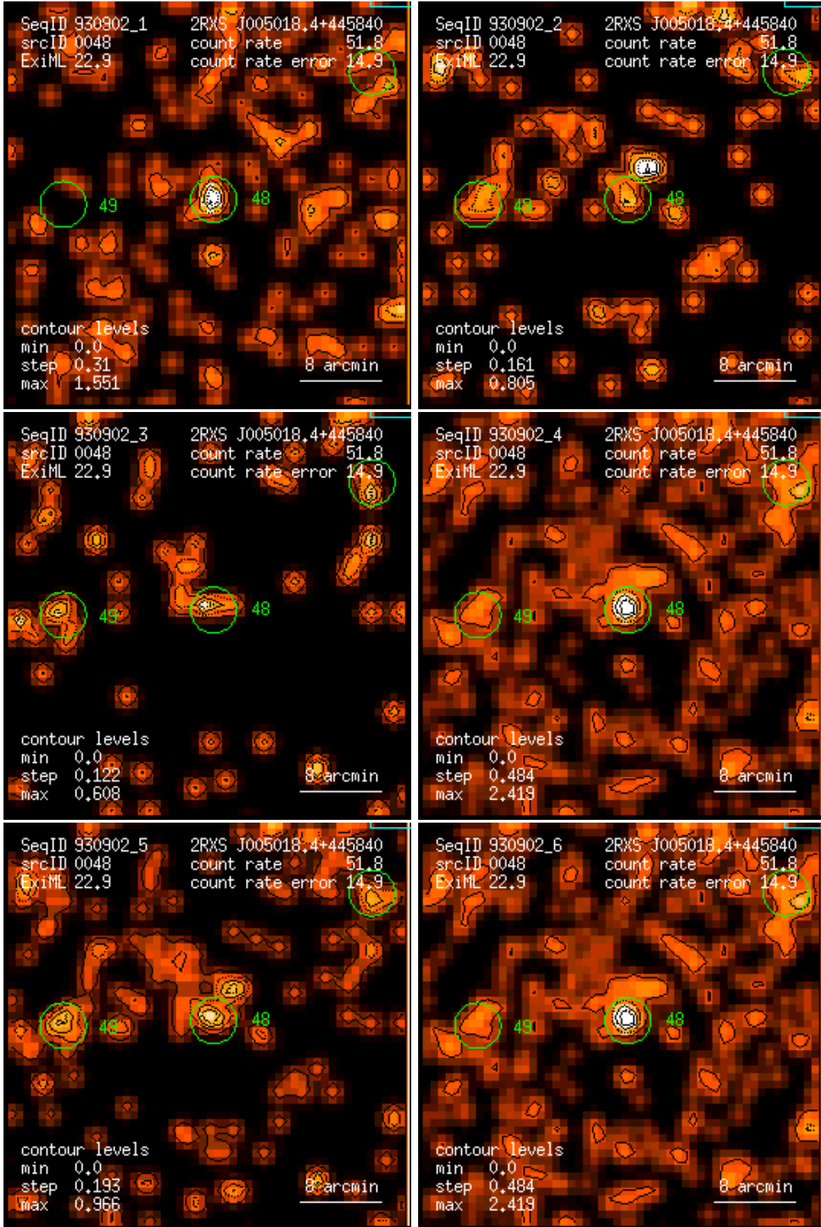
Figure 48: RASS 930902: detection 0048: band rate images, Gaussian filter: (1) PSPC channels 11 – 41, (2) 52 – 90, (3) 91 – 201, (4) 11 – 235, (5) 52 – 201, (6) 11 – 201. Broad band rates in counts/ks. Band rate contour levels in counts/ks/arcmin 2 .
