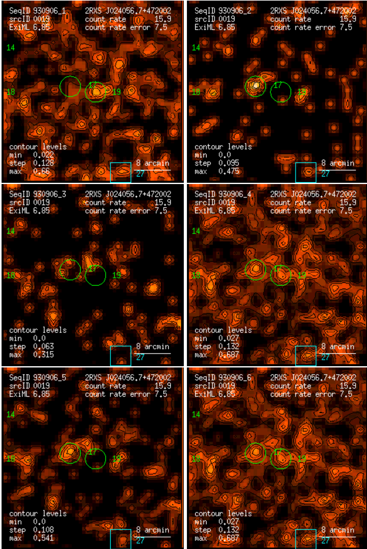
Figure 19: RASS 930906: detection 0019: band rate images, Gaussian filter: (1) PSPC channels 11 – 41, (2) 52 – 90, (3) 91 – 201, (4) 11 – 235, (5) 52 – 201, (6) 11 – 201. Broad band rates in counts/ks. Band rate contour levels in counts/ks/arcmin 2 .
