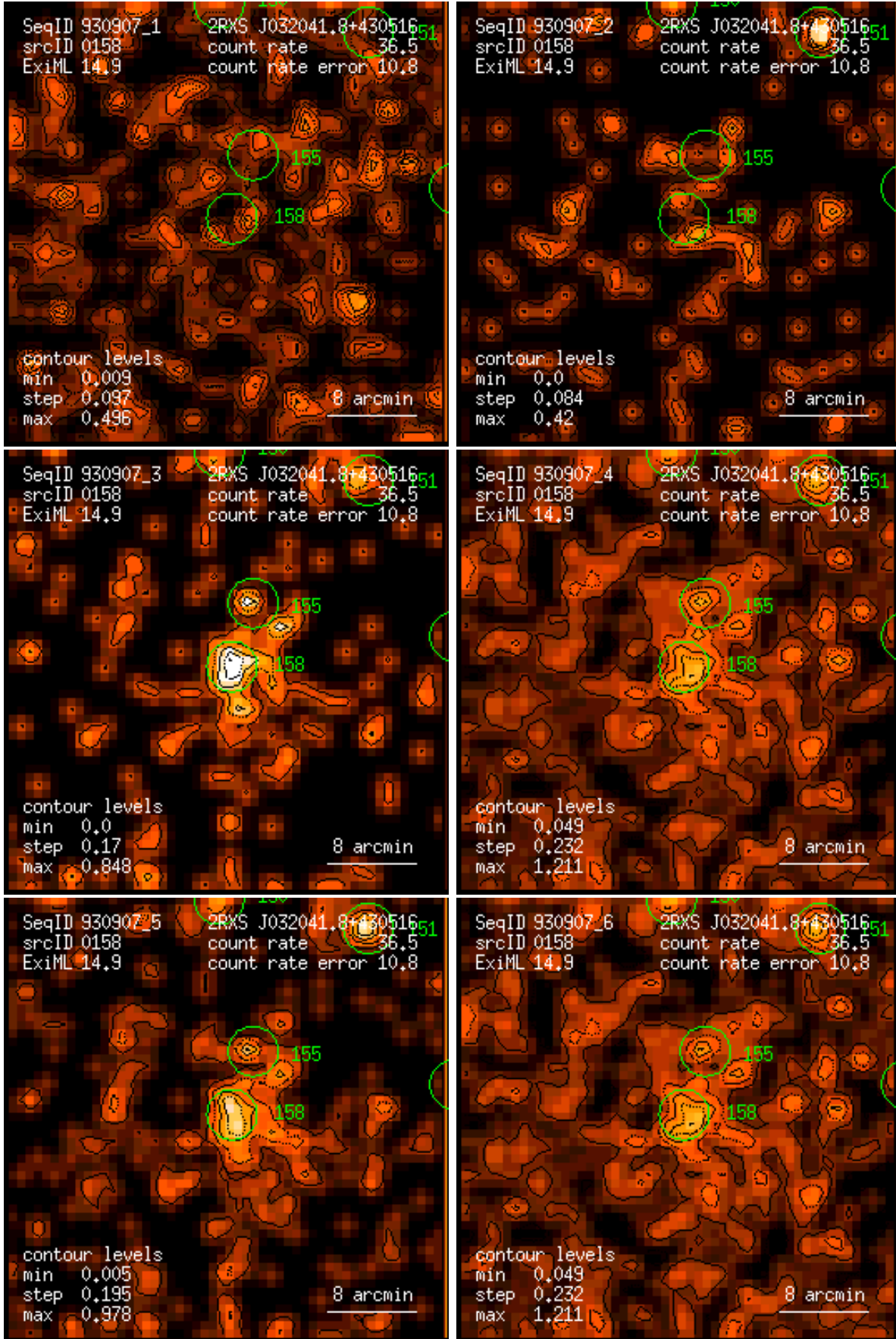
Figure 158: RASS 930907: detection 0158: band rate images, Gaussian filter: (1) PSPC channels 11 – 41, (2) 52 – 90, (3) 91 – 201, (4) 11 – 235, (5) 52 – 201, (6) 11 – 201. Broad band rates in counts/ks. Band rate contour levels in counts/ks/arcmin 2 .
