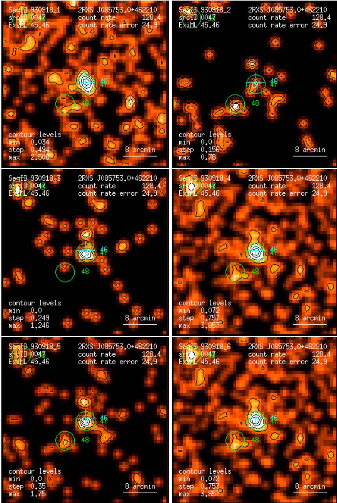
Figure 47: RASS 930918: detection 0047: band rate images, Gaussian filter: (1) PSPC channels 11 – 41, (2) 52 – 90, (3) 91 – 201, (4) 11 – 235, (5) 52 – 201, (6) 11 – 201. Broad band rates in counts/ks. Band rate contour levels in counts/ks/arcmin 2 .
