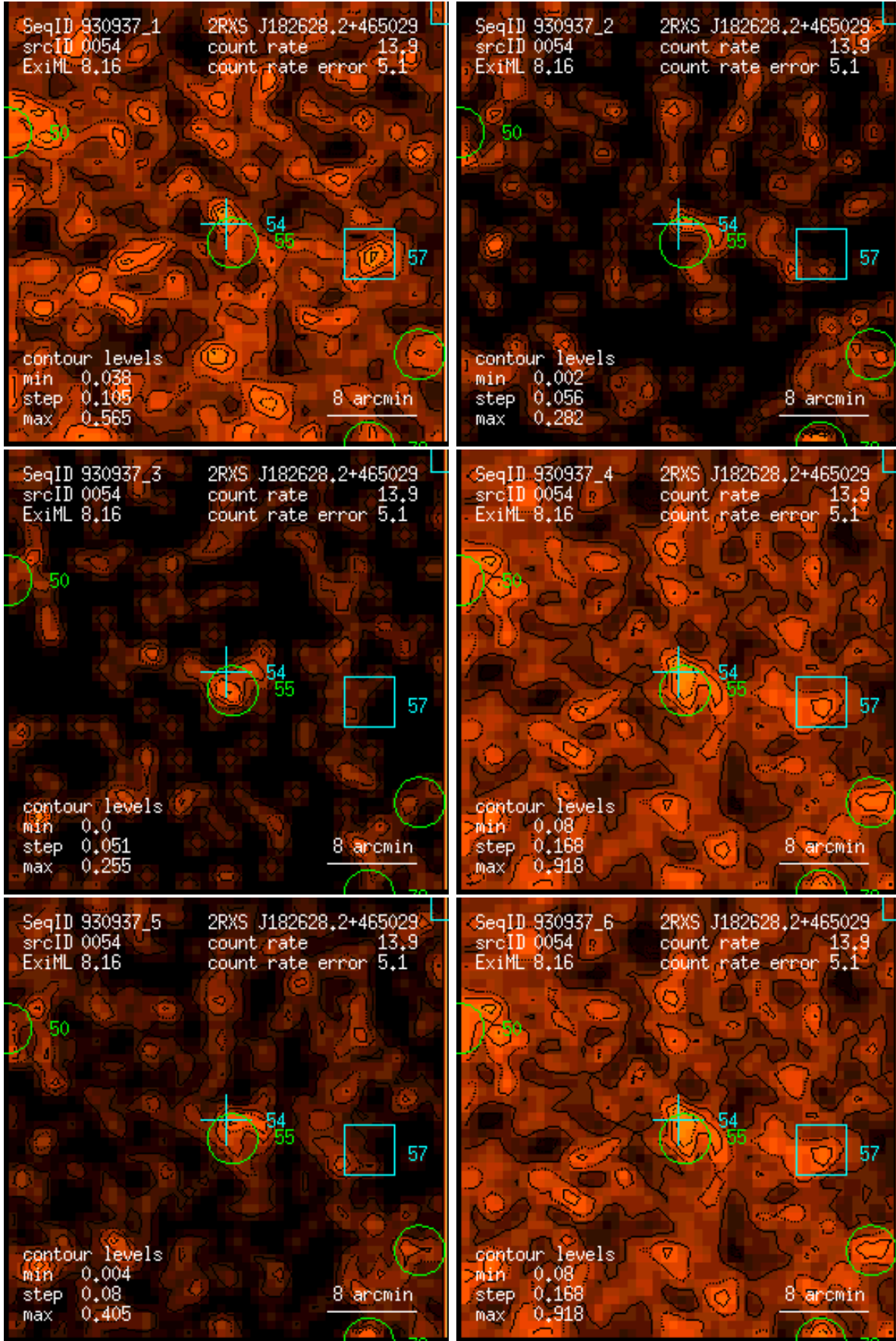
Figure 54: RASS 930937: detection 0054: band rate images, Gaussian filter: (1) PSPC channels 11 – 41, (2) 52 – 90, (3) 91 – 201, (4) 11 – 235, (5) 52 – 201, (6) 11 – 201. Broad band rates in counts/ks. Band rate contour levels in counts/ks/arcmin 2 .
