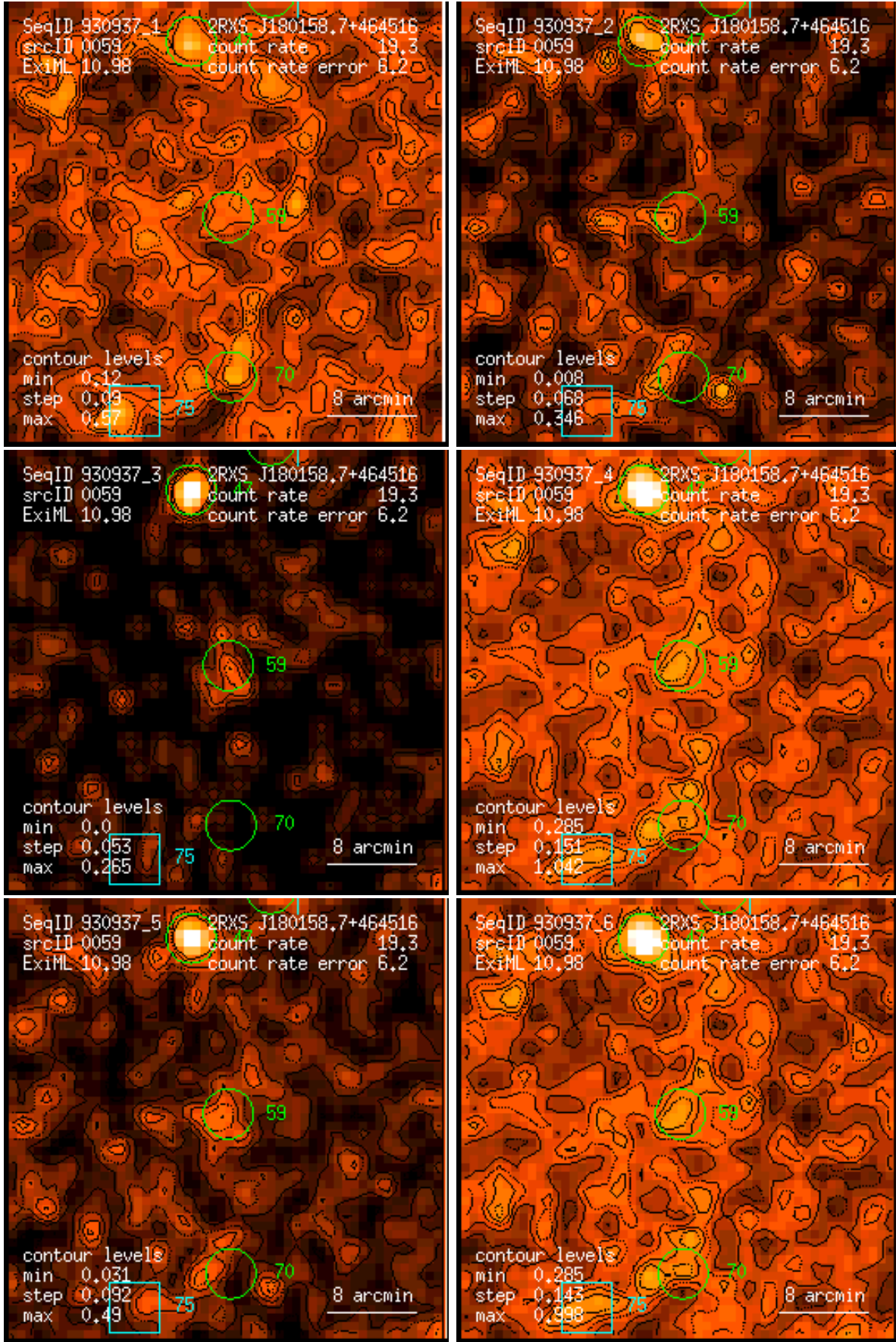
Figure 59: RASS 930937: detection 0059: band rate images, Gaussian filter: (1) PSPC channels 11 – 41, (2) 52 – 90, (3) 91 – 201, (4) 11 – 235, (5) 52 – 201, (6) 11 – 201. Broad band rates in counts/ks. Band rate contour levels in counts/ks/arcmin 2 .
