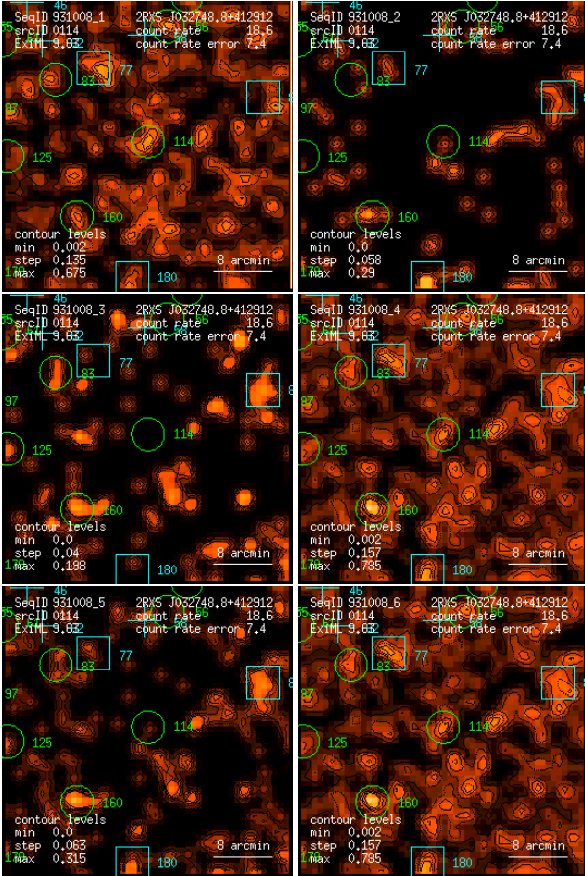
Figure 114: RASS 931008: detection 0114: band rate images, Gaussian filter: (1) PSPC channels 11 – 41, (2) 52 – 90, (3) 91 – 201, (4) 11 – 235, (5) 52 – 201, (6) 11 – 201. Broad band rates in counts/ks. Band rate contour levels in counts/ks/arcmin 2 .
