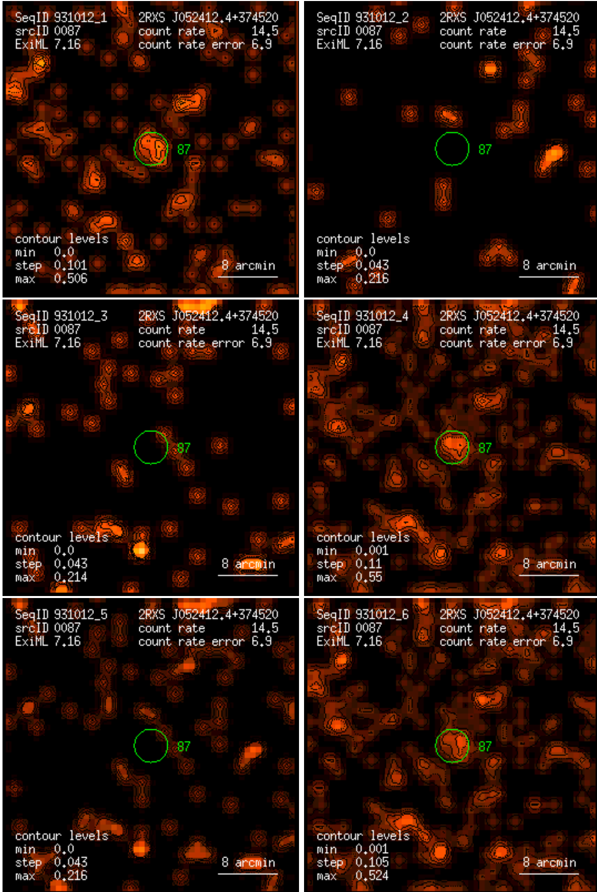
Figure 87: RASS 931012: detection 0087: band rate images, Gaussian filter: (1) PSPC channels 11 – 41, (2) 52 – 90, (3) 91 – 201, (4) 11 – 235, (5) 52 – 201, (6) 11 – 201. Broad band rates in counts/ks. Band rate contour levels in counts/ks/arcmin 2 .
