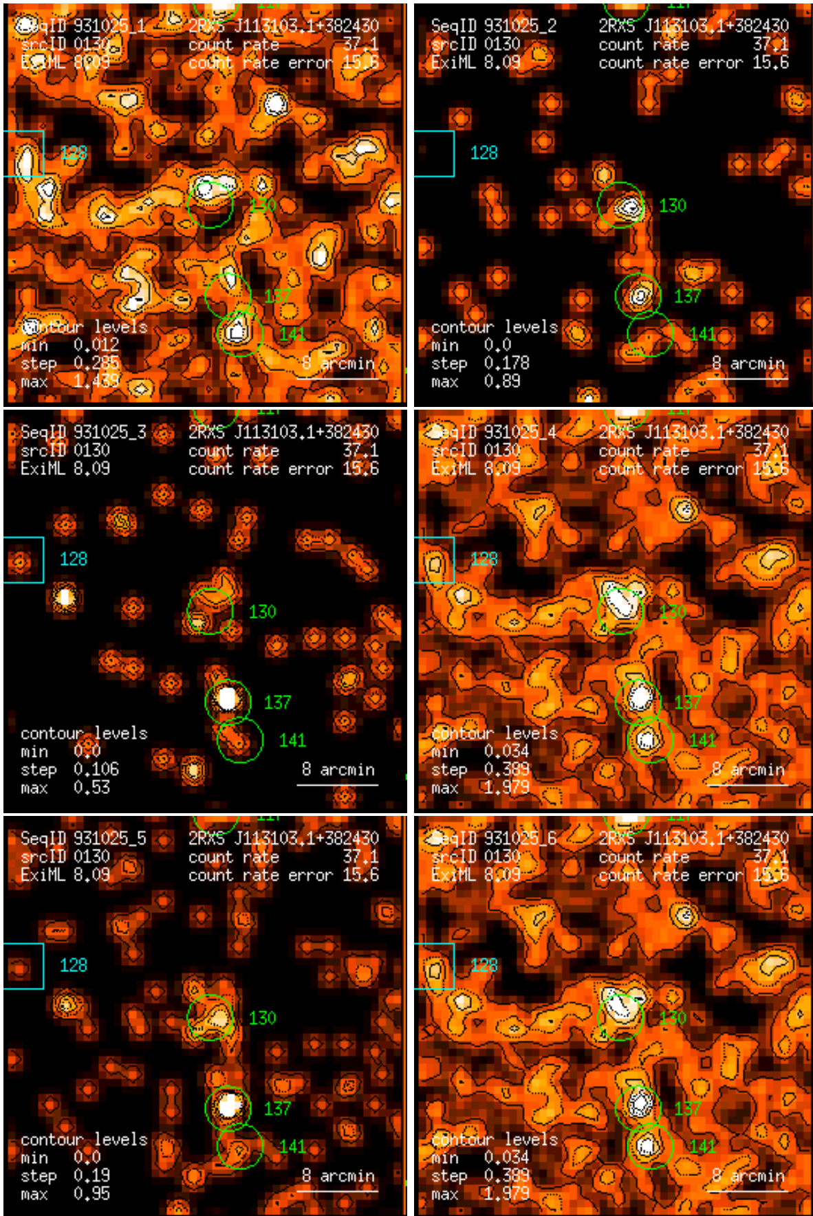
Figure 130: RASS 931025: detection 0130: band rate images, Gaussian filter: (1) PSPC channels 11 – 41, (2) 52 – 90, (3) 91 – 201, (4) 11 – 235, (5) 52 – 201, (6) 11 – 201. Broad band rates in counts/ks. Band rate contour levels in counts/ks/arcmin 2 .
