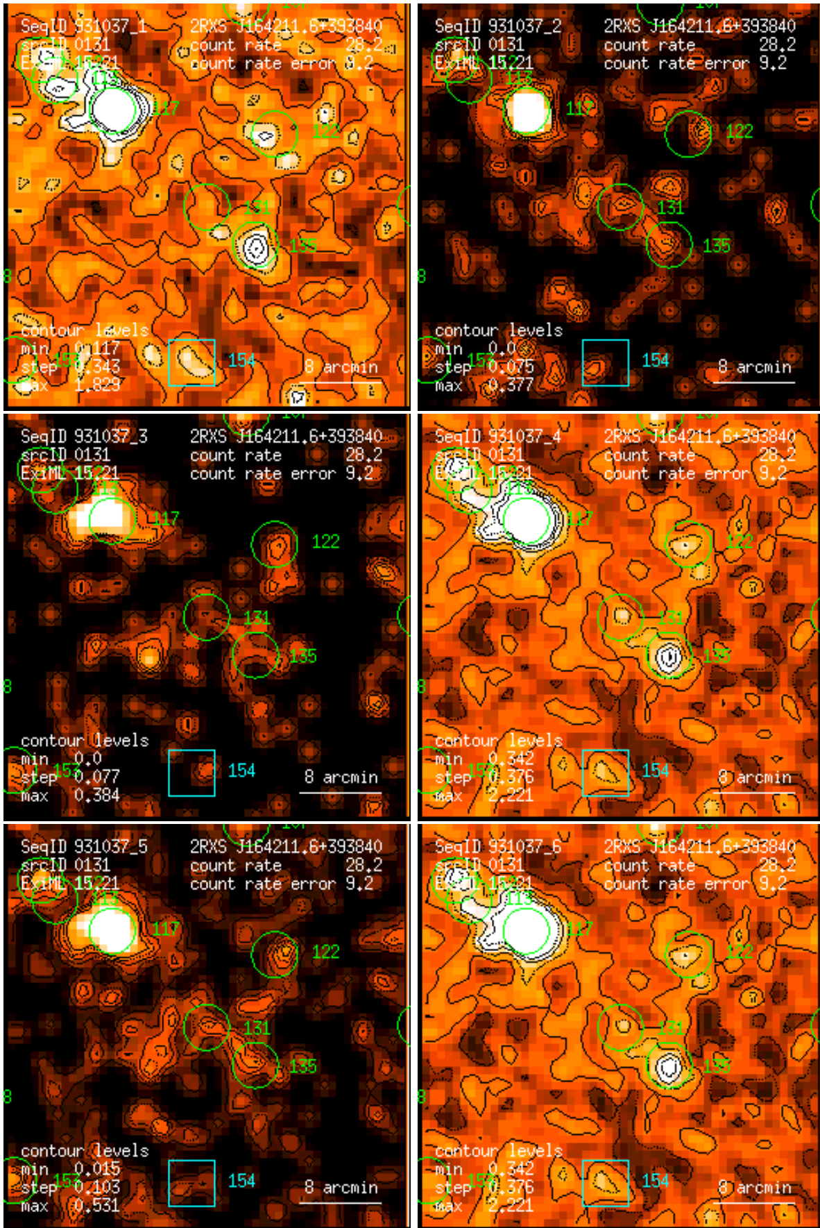
Figure 131: RASS 931037: detection 0131: band rate images, Gaussian filter: (1) PSPC channels 11 – 41, (2) 52 – 90, (3) 91 – 201, (4) 11 – 235, (5) 52 – 201, (6) 11 – 201. Broad band rates in counts/ks. Band rate contour levels in counts/ks/arcmin 2 .
