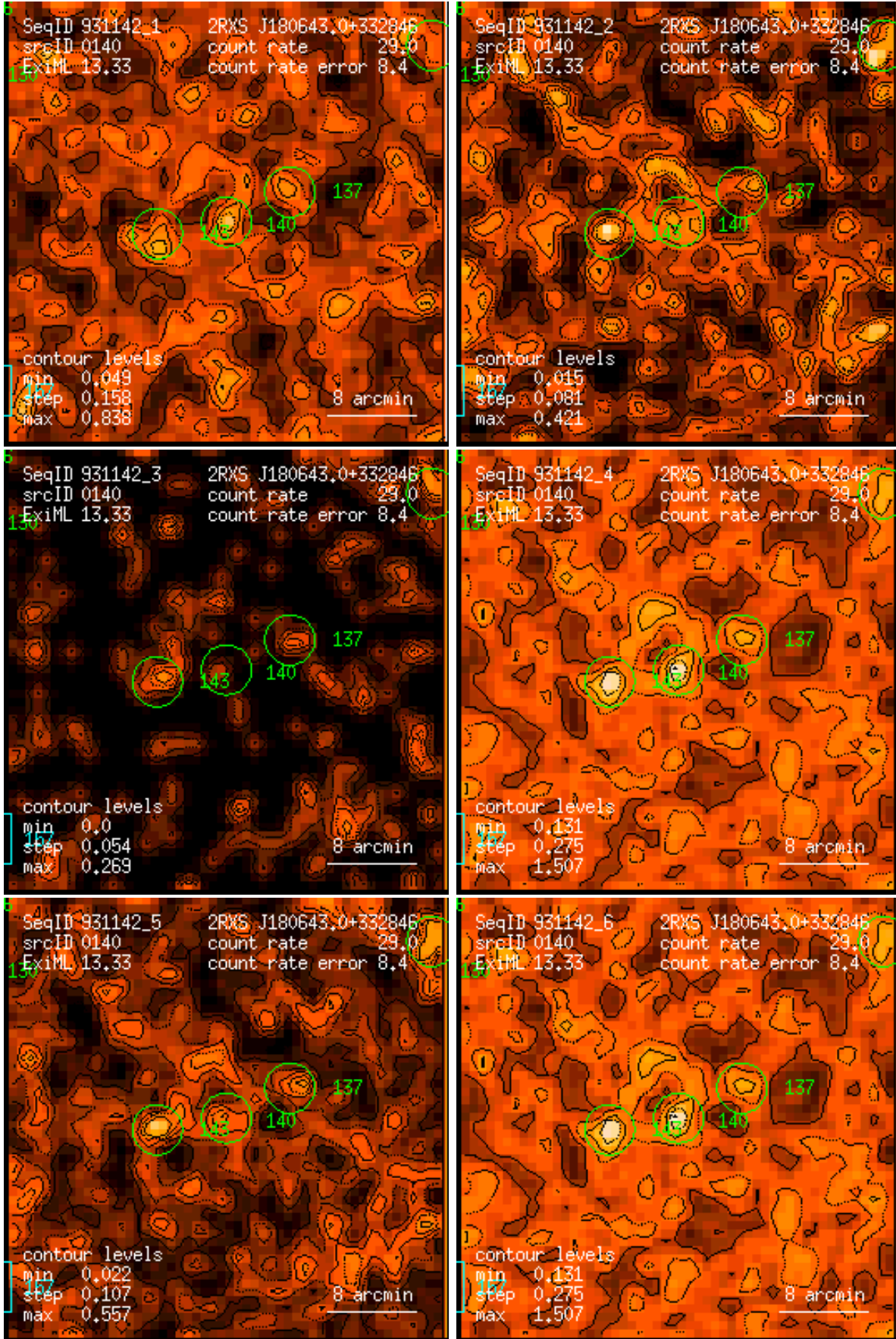
Figure 140: RASS 931142: detection 0140: band rate images, Gaussian filter: (1) PSPC channels 11 – 41, (2) 52 – 90, (3) 91 – 201, (4) 11 – 235, (5) 52 – 201, (6) 11 – 201. Broad band rates in counts/ks. Band rate contour levels in counts/ks/arcmin 2 .
