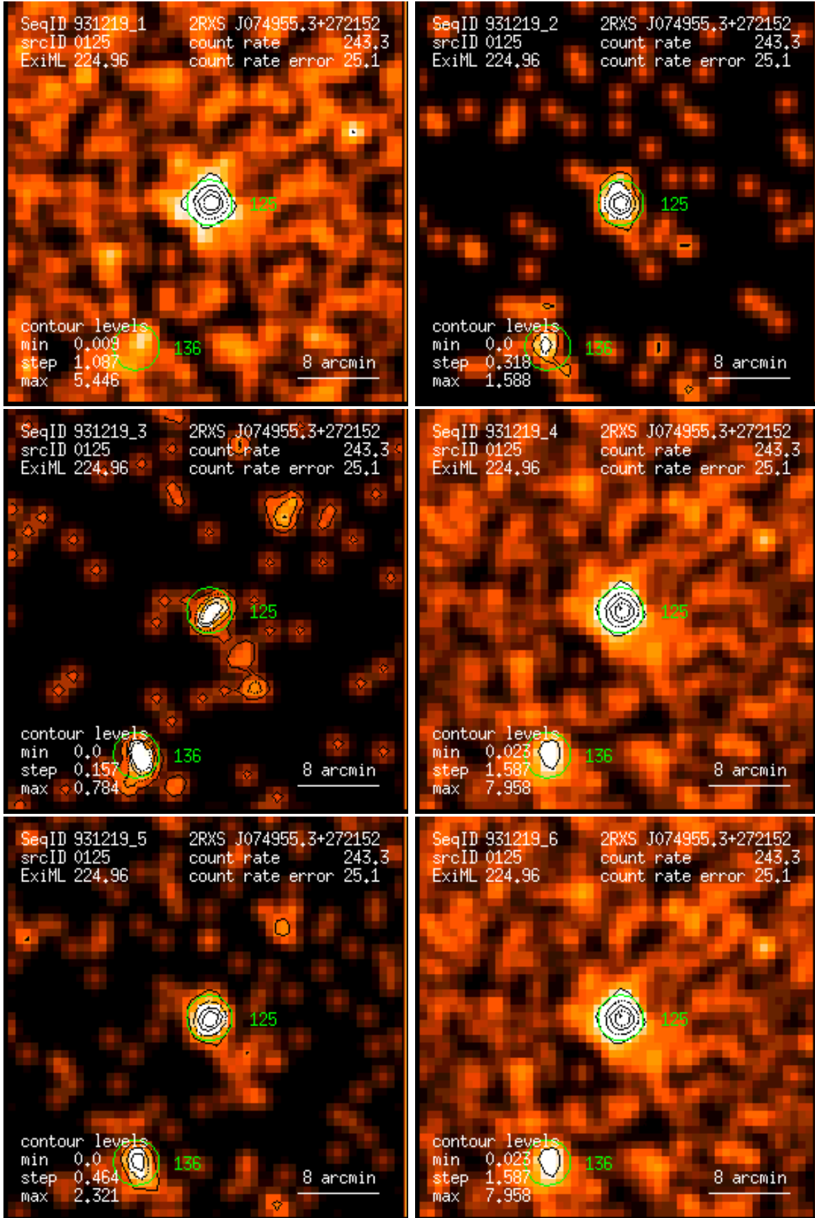
Figure 125: RASS 931219: detection 0125: band rate images, Gaussian filter: (1) PSPC channels 11 – 41, (2) 52 – 90, (3) 91 – 201, (4) 11 – 235, (5) 52 – 201, (6) 11 – 201. Broad band rates in counts/ks. Band rate contour levels in counts/ks/arcmin 2 .
