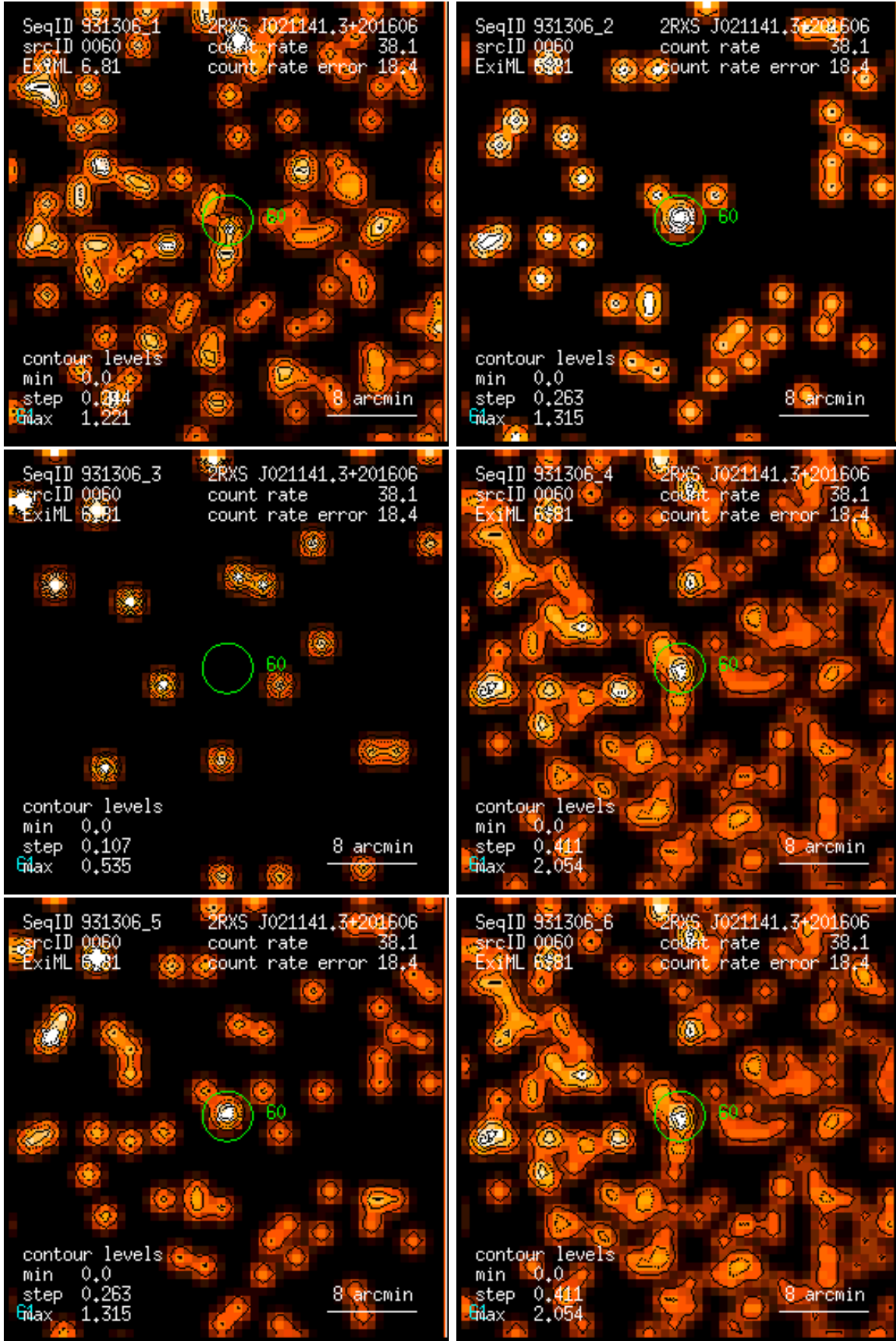
Figure 60: RASS 931306: detection 0060: band rate images, Gaussian filter: (1) PSPC channels 11 – 41, (2) 52 – 90, (3) 91 – 201, (4) 11 – 235, (5) 52 – 201, (6) 11 – 201. Broad band rates in counts/ks. Band rate contour levels in counts/ks/arcmin 2 .
