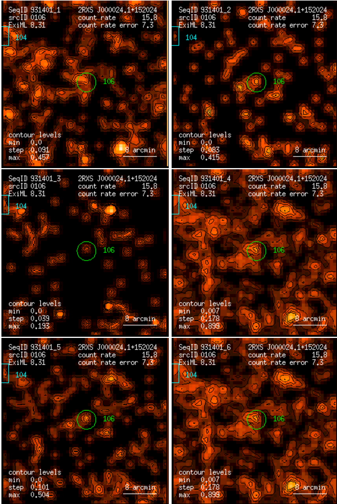
Figure 106: RASS 931401: detection 0106: band rate images, Gaussian filter: (1) PSPC channels 11 – 41, (2) 52 – 90, (3) 91 – 201, (4) 11 – 235, (5) 52 – 201, (6) 11 – 201. Broad band rates in counts/ks. Band rate contour levels in counts/ks/arcmin 2 .
