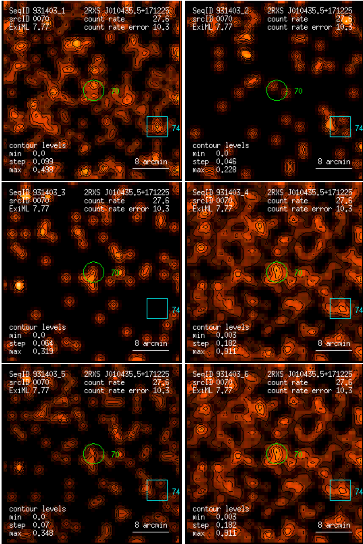
Figure 70: RASS 931403: detection 0070: band rate images, Gaussian filter: (1) PSPC channels 11 – 41, (2) 52 – 90, (3) 91 – 201, (4) 11 – 235, (5) 52 – 201, (6) 11 – 201. Broad band rates in counts/ks. Band rate contour levels in counts/ks/arcmin 2 .
