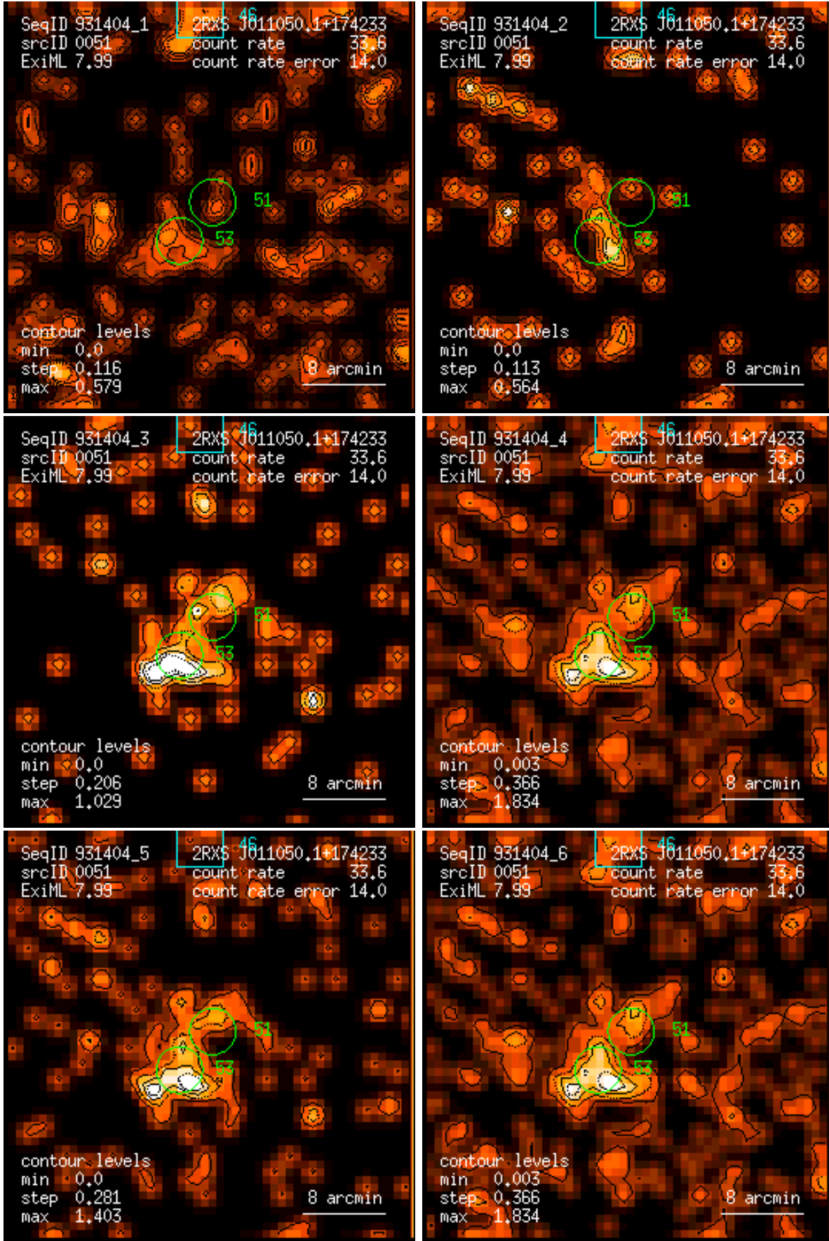
Figure 51: RASS 931404: detection 0051: band rate images, Gaussian filter: (1) PSPC channels 11 – 41, (2) 52 – 90, (3) 91 – 201, (4) 11 – 235, (5) 52 – 201, (6) 11 – 201. Broad band rates in counts/ks. Band rate contour levels in counts/ks/arcmin 2 .
