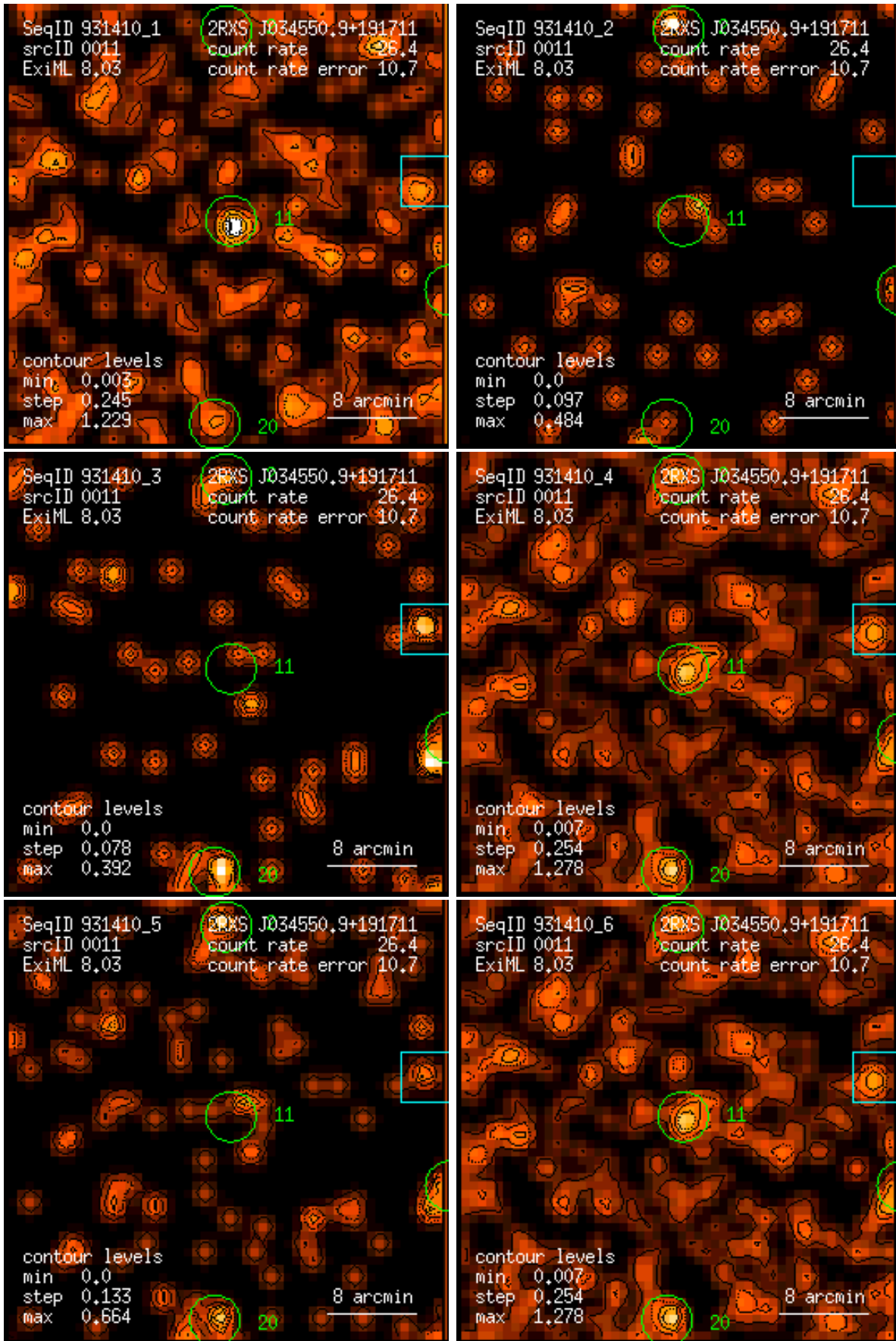
Figure 11: RASS 931410: detection 0011: band rate images, Gaussian filter: (1) PSPC channels 11 – 41, (2) 52 – 90, (3) 91 – 201, (4) 11 – 235, (5) 52 – 201, (6) 11 – 201. Broad band rates in counts/ks. Band rate contour levels in counts/ks/arcmin 2 .
