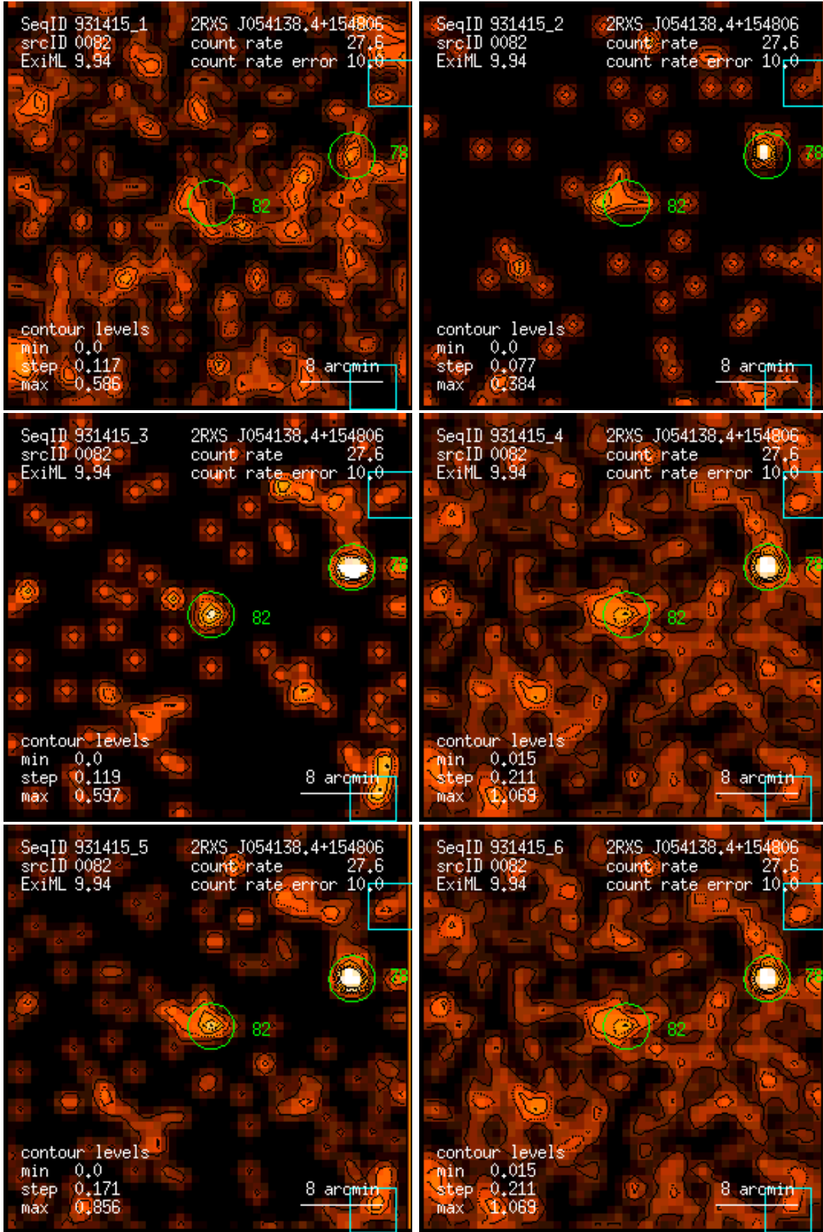
Figure 82: RASS 931415: detection 0082: band rate images, Gaussian filter: (1) PSPC channels 11 – 41, (2) 52 – 90, (3) 91 – 201, (4) 11 – 235, (5) 52 – 201, (6) 11 – 201. Broad band rates in counts/ks. Band rate contour levels in counts/ks/arcmin 2 .
