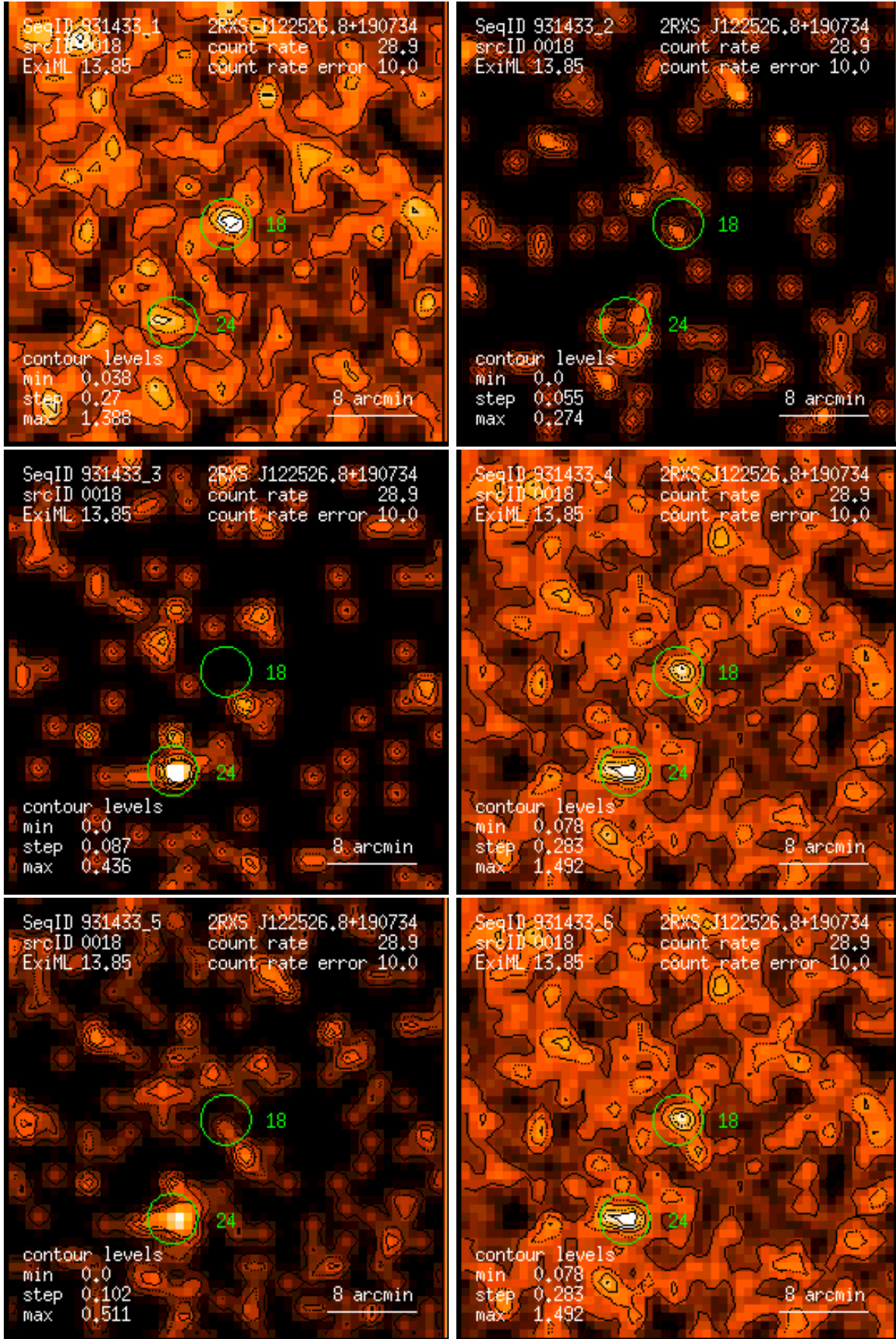
Figure 18: RASS 931433: detection 0018: band rate images, Gaussian filter: (1) PSPC channels 11 – 41, (2) 52 – 90, (3) 91 – 201, (4) 11 – 235, (5) 52 – 201, (6) 11 – 201. Broad band rates in counts/ks. Band rate contour levels in counts/ks/arcmin 2 .
