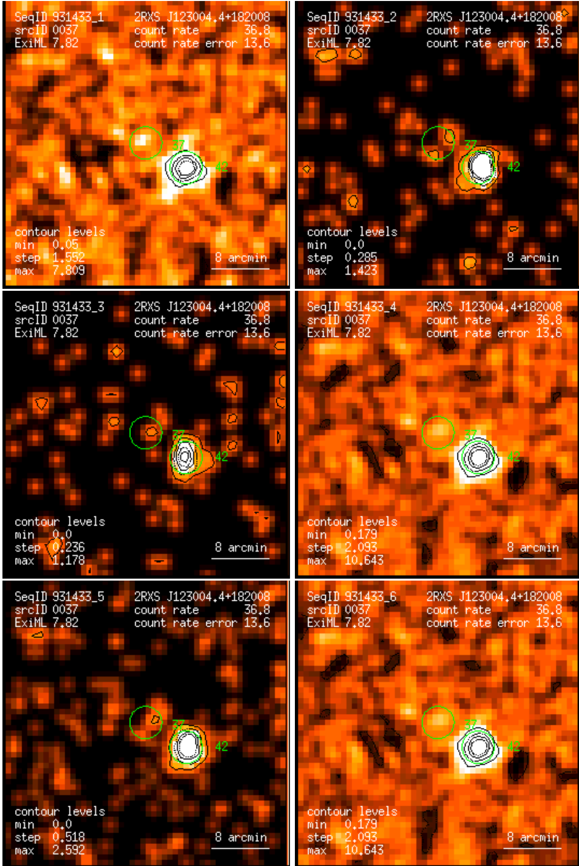
Figure 37: RASS 931433: detection 0037: band rate images, Gaussian filter: (1) PSPC channels 11 – 41, (2) 52 – 90, (3) 91 – 201, (4) 11 – 235, (5) 52 – 201, (6) 11 – 201. Broad band rates in counts/ks. Band rate contour levels in counts/ks/arcmin 2 .
