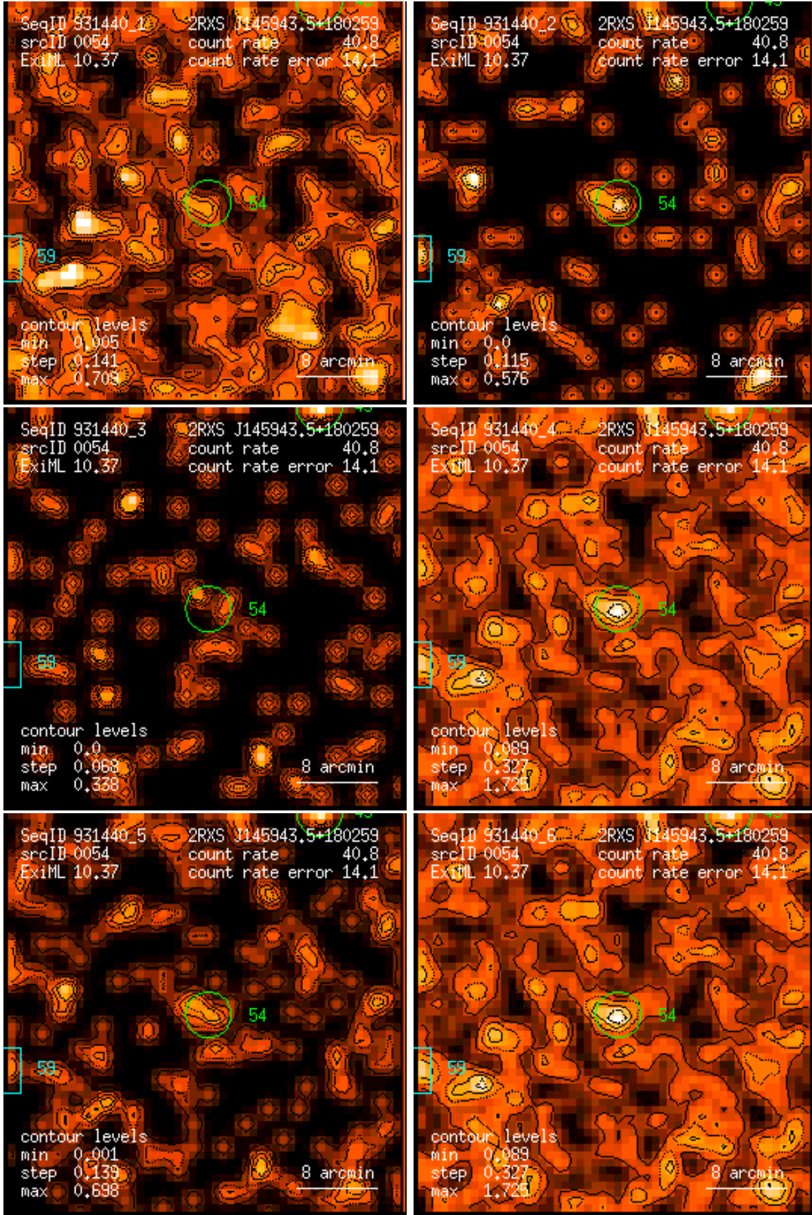
Figure 54: RASS 931440: detection 0054: band rate images, Gaussian filter: (1) PSPC channels 11 – 41, (2) 52 – 90, (3) 91 – 201, (4) 11 – 235, (5) 52 – 201, (6) 11 – 201. Broad band rates in counts/ks. Band rate contour levels in counts/ks/arcmin 2 .
