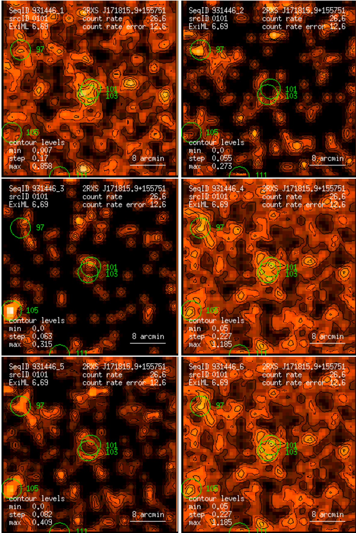
Figure 101: RASS 931446: detection 0101: band rate images, Gaussian filter: (1) PSPC channels 11 – 41, (2) 52 – 90, (3) 91 – 201, (4) 11 – 235, (5) 52 – 201, (6) 11 – 201. Broad band rates in counts/ks. Band rate contour levels in counts/ks/arcmin 2 .
