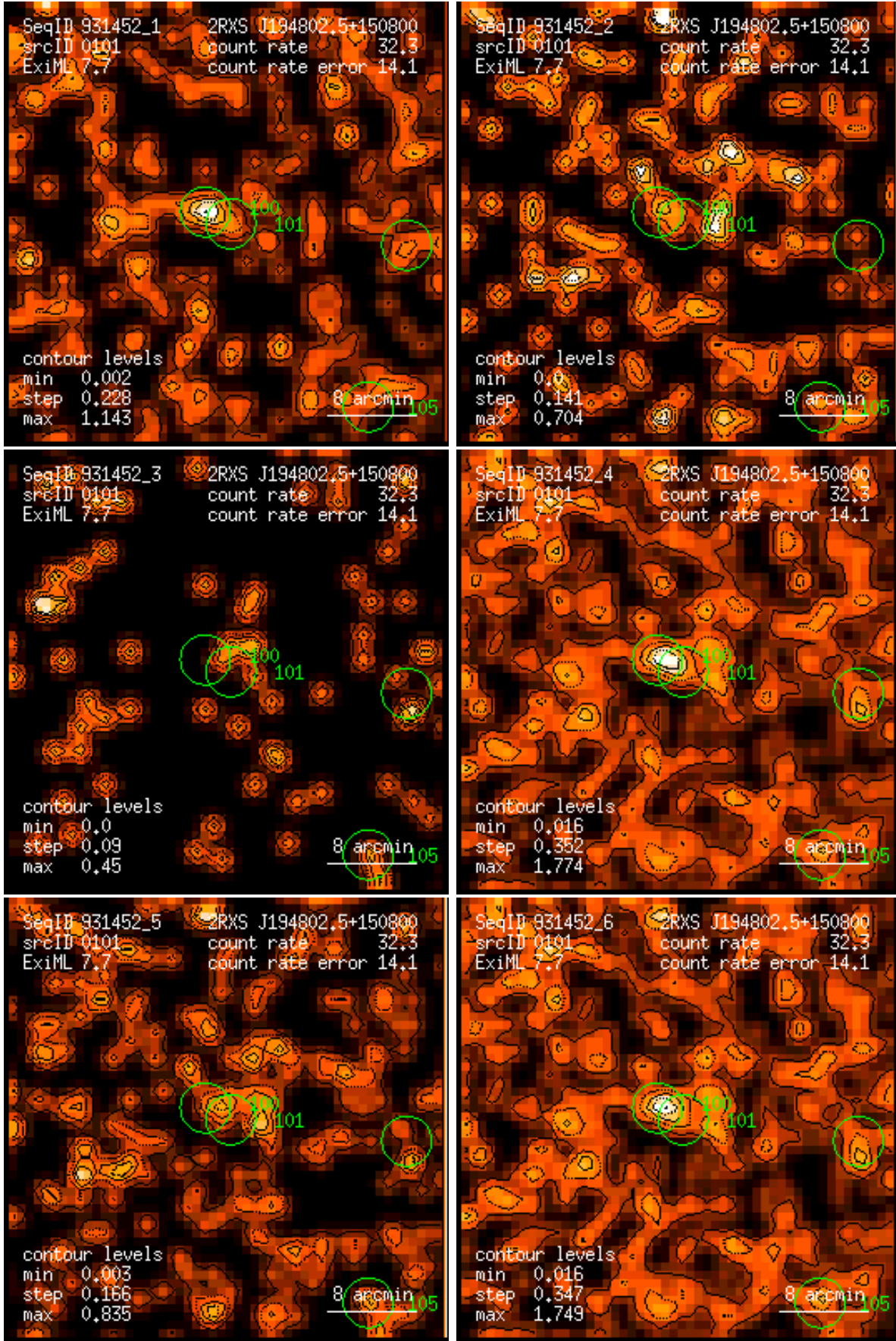
Figure 101: RASS 931452: detection 0101: band rate images, Gaussian filter: (1) PSPC channels 11 – 41, (2) 52 – 90, (3) 91 – 201, (4) 11 – 235, (5) 52 – 201, (6) 11 – 201. Broad band rates in counts/ks. Band rate contour levels in counts/ks/arcmin 2 .
