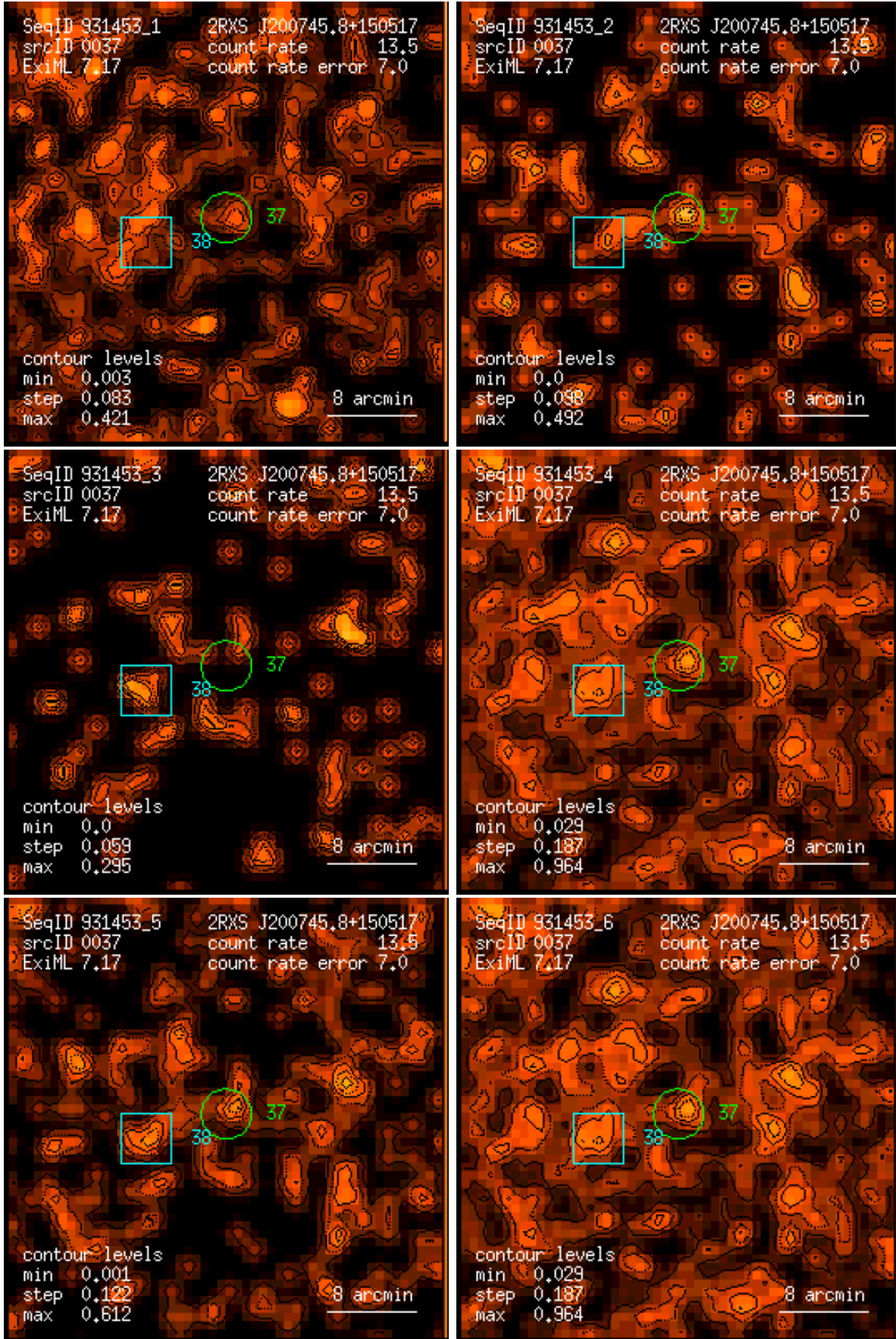
Figure 37: RASS 931453: detection 0037: band rate images, Gaussian filter: (1) PSPC channels 11 – 41, (2) 52 – 90, (3) 91 – 201, (4) 11 – 235, (5) 52 – 201, (6) 11 – 201. Broad band rates in counts/ks. Band rate contour levels in counts/ks/arcmin 2 .
