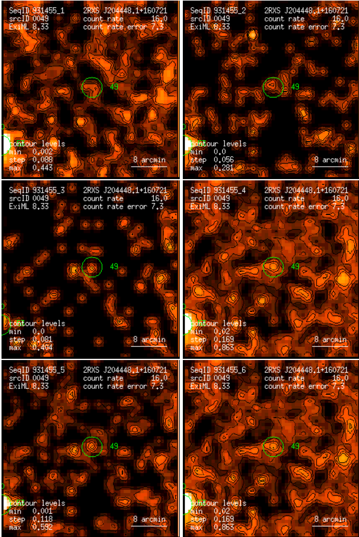
Figure 49: RASS 931455: detection 0049: band rate images, Gaussian filter: (1) PSPC channels 11 – 41, (2) 52 – 90, (3) 91 – 201, (4) 11 – 235, (5) 52 – 201, (6) 11 – 201. Broad band rates in counts/ks. Band rate contour levels in counts/ks/arcmin 2 .
