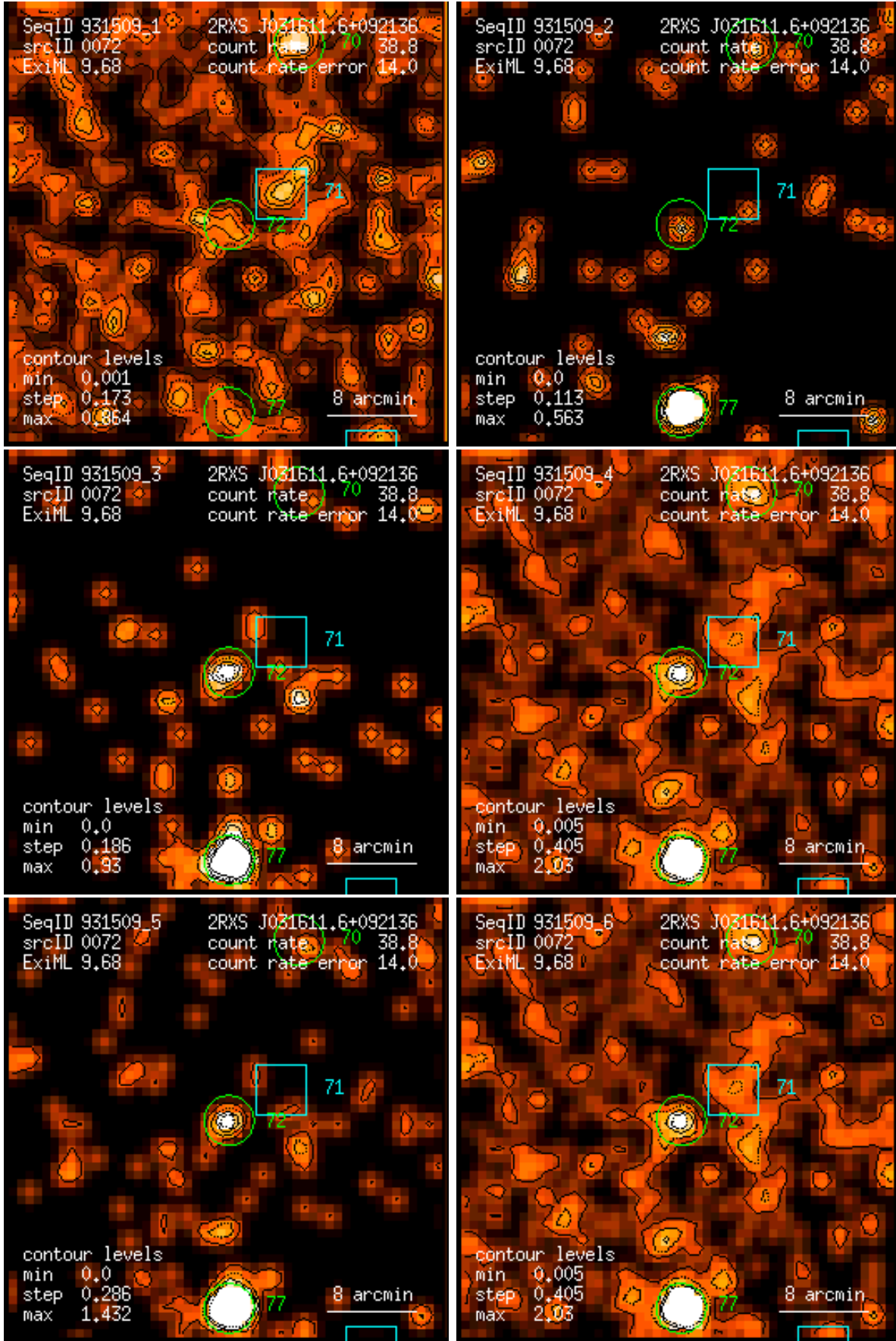
Figure 72: RASS 931509: detection 0072: band rate images, Gaussian filter: (1) PSPC channels 11 – 41, (2) 52 – 90, (3) 91 – 201, (4) 11 – 235, (5) 52 – 201, (6) 11 – 201. Broad band rates in counts/ks. Band rate contour levels in counts/ks/arcmin 2 .
