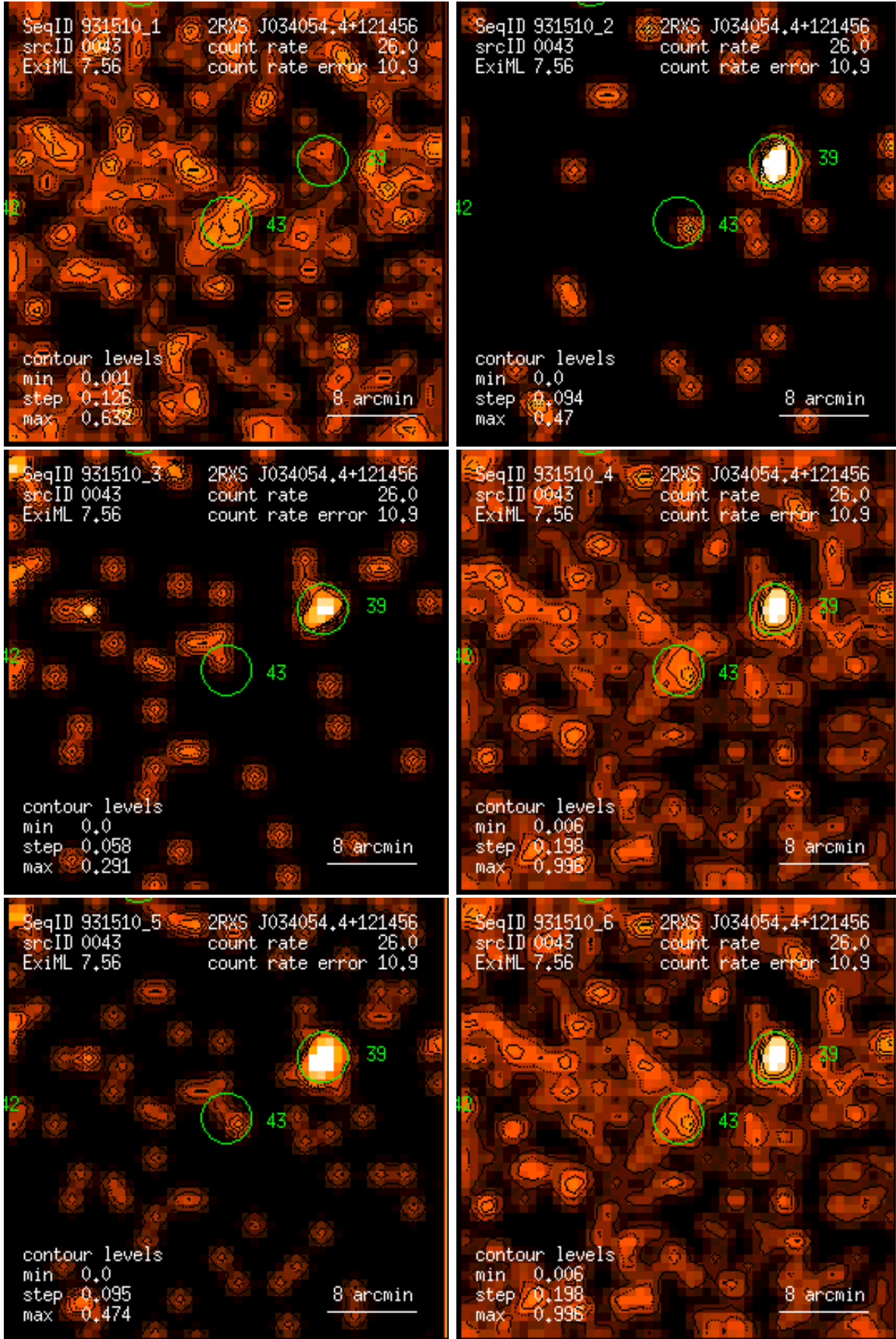
Figure 43: RASS 931510: detection 0043: band rate images, Gaussian filter: (1) PSPC channels 11 – 41, (2) 52 – 90, (3) 91 – 201, (4) 11 – 235, (5) 52 – 201, (6) 11 – 201. Broad band rates in counts/ks. Band rate contour levels in counts/ks/arcmin 2 .
