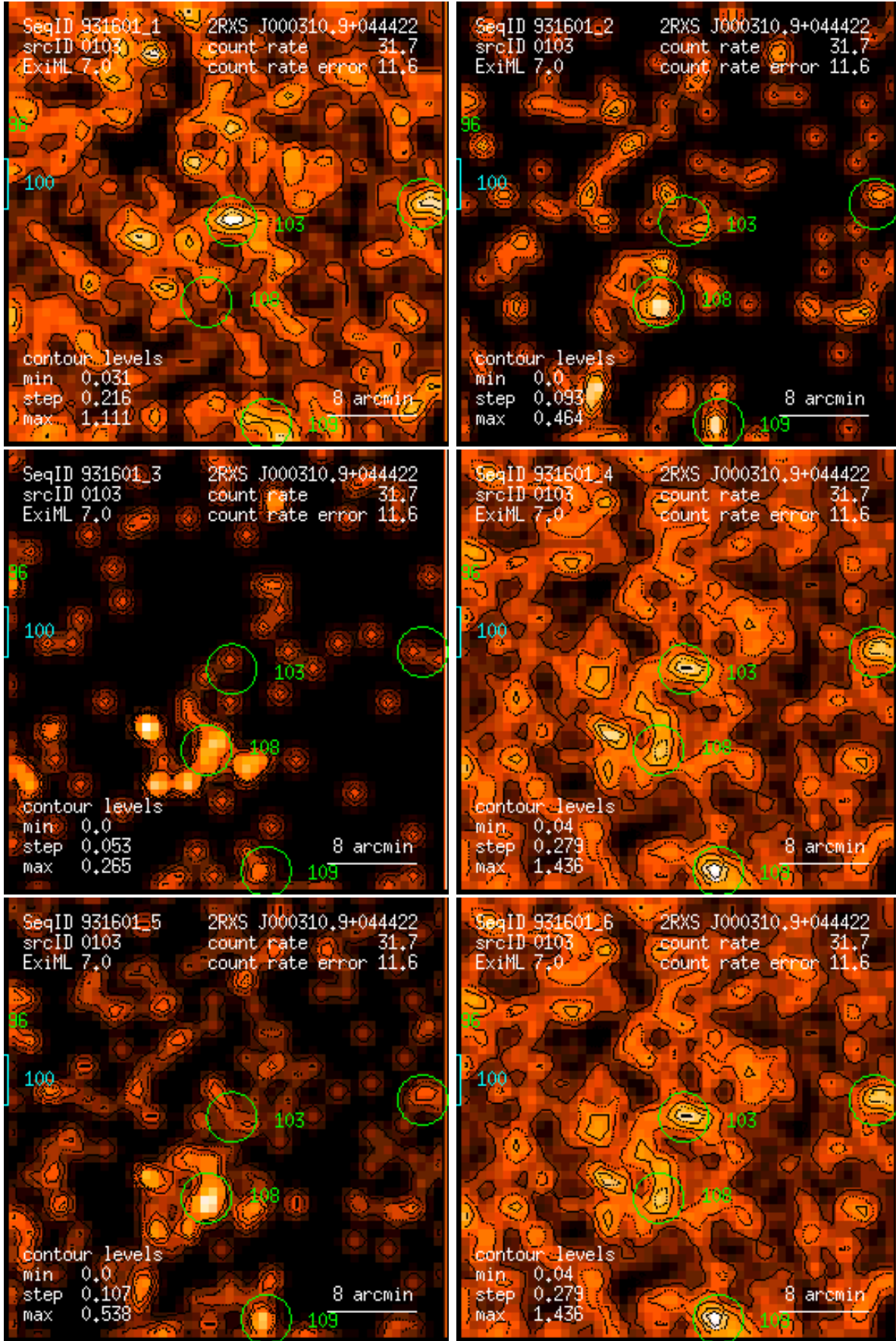
Figure 103: RASS 931601: detection 0103: band rate images, Gaussian filter: (1) PSPC channels 11 – 41, (2) 52 – 90, (3) 91 – 201, (4) 11 – 235, (5) 52 – 201, (6) 11 – 201. Broad band rates in counts/ks. Band rate contour levels in counts/ks/arcmin 2 .
