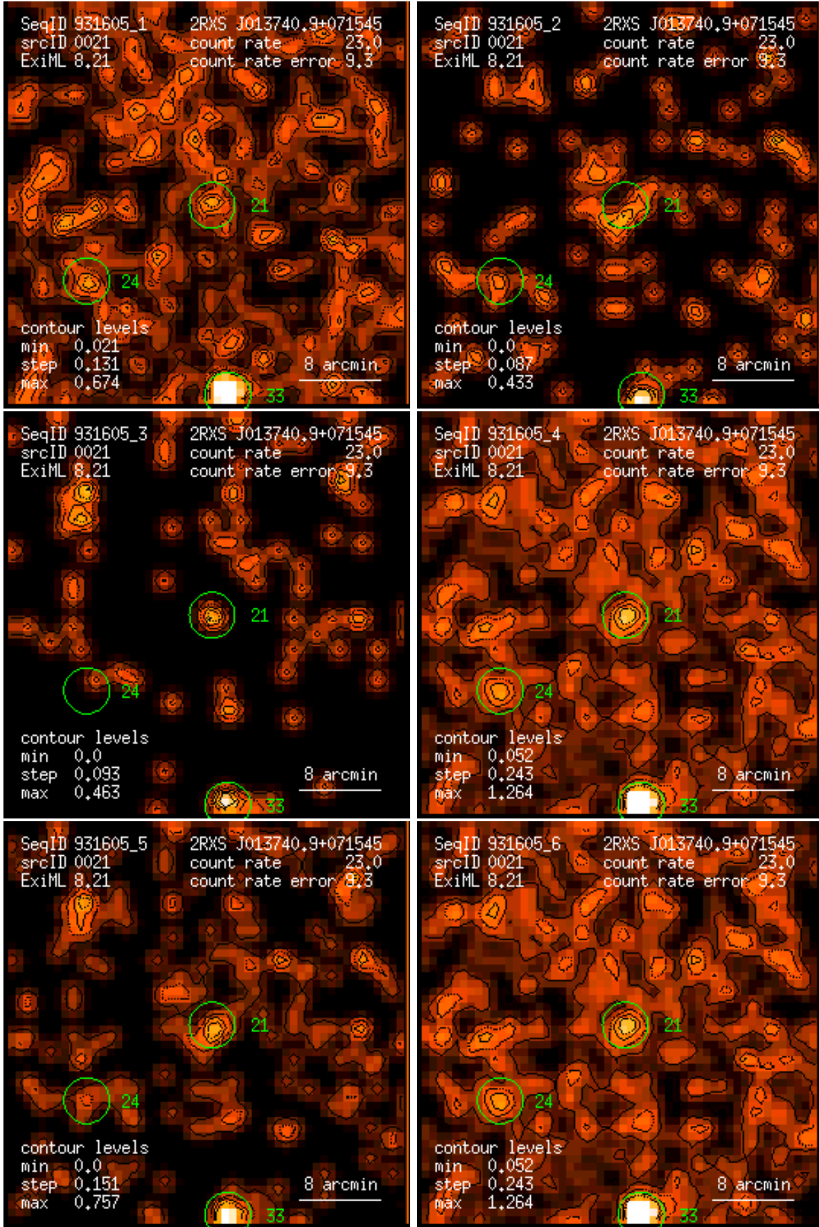
Figure 21: RASS 931605: detection 0021: band rate images, Gaussian filter: (1) PSPC channels 11 – 41, (2) 52 – 90, (3) 91 – 201, (4) 11 – 235, (5) 52 – 201, (6) 11 – 201. Broad band rates in counts/ks. Band rate contour levels in counts/ks/arcmin 2 .
