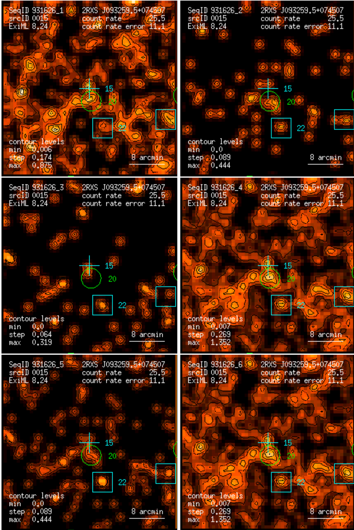
Figure 15: RASS 931626: detection 0015: band rate images, Gaussian filter: (1) PSPC channels 11 – 41, (2) 52 – 90, (3) 91 – 201, (4) 11 – 235, (5) 52 – 201, (6) 11 – 201. Broad band rates in counts/ks. Band rate contour levels in counts/ks/arcmin 2 .
