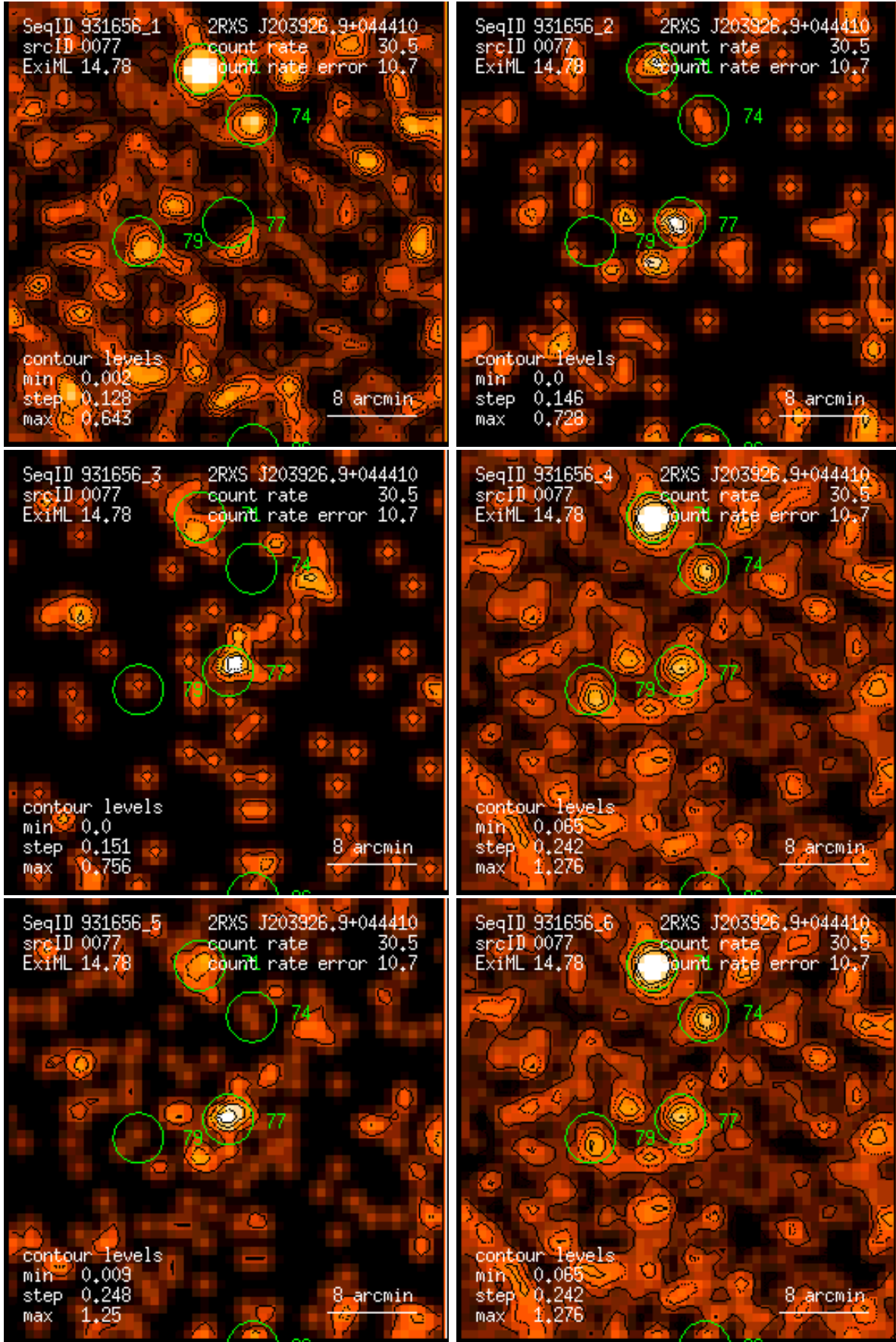
Figure 77: RASS 931656: detection 0077: band rate images, Gaussian filter: (1) PSPC channels 11 – 41, (2) 52 – 90, (3) 91 – 201, (4) 11 – 235, (5) 52 – 201, (6) 11 – 201. Broad band rates in counts/ks. Band rate contour levels in counts/ks/arcmin 2 .
