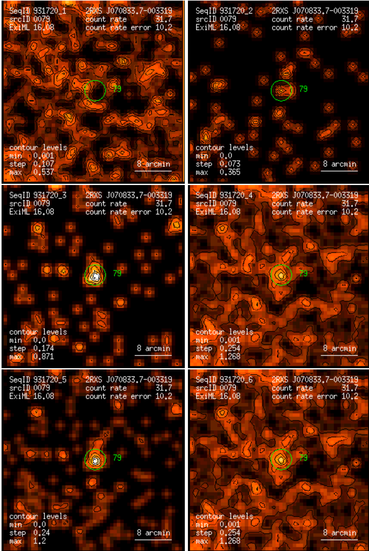
Figure 79: RASS 931720: detection 0079: band rate images, Gaussian filter: (1) PSPC channels 11 – 41, (2) 52 – 90, (3) 91 – 201, (4) 11 – 235, (5) 52 – 201, (6) 11 – 201. Broad band rates in counts/ks. Band rate contour levels in counts/ks/arcmin 2 .
