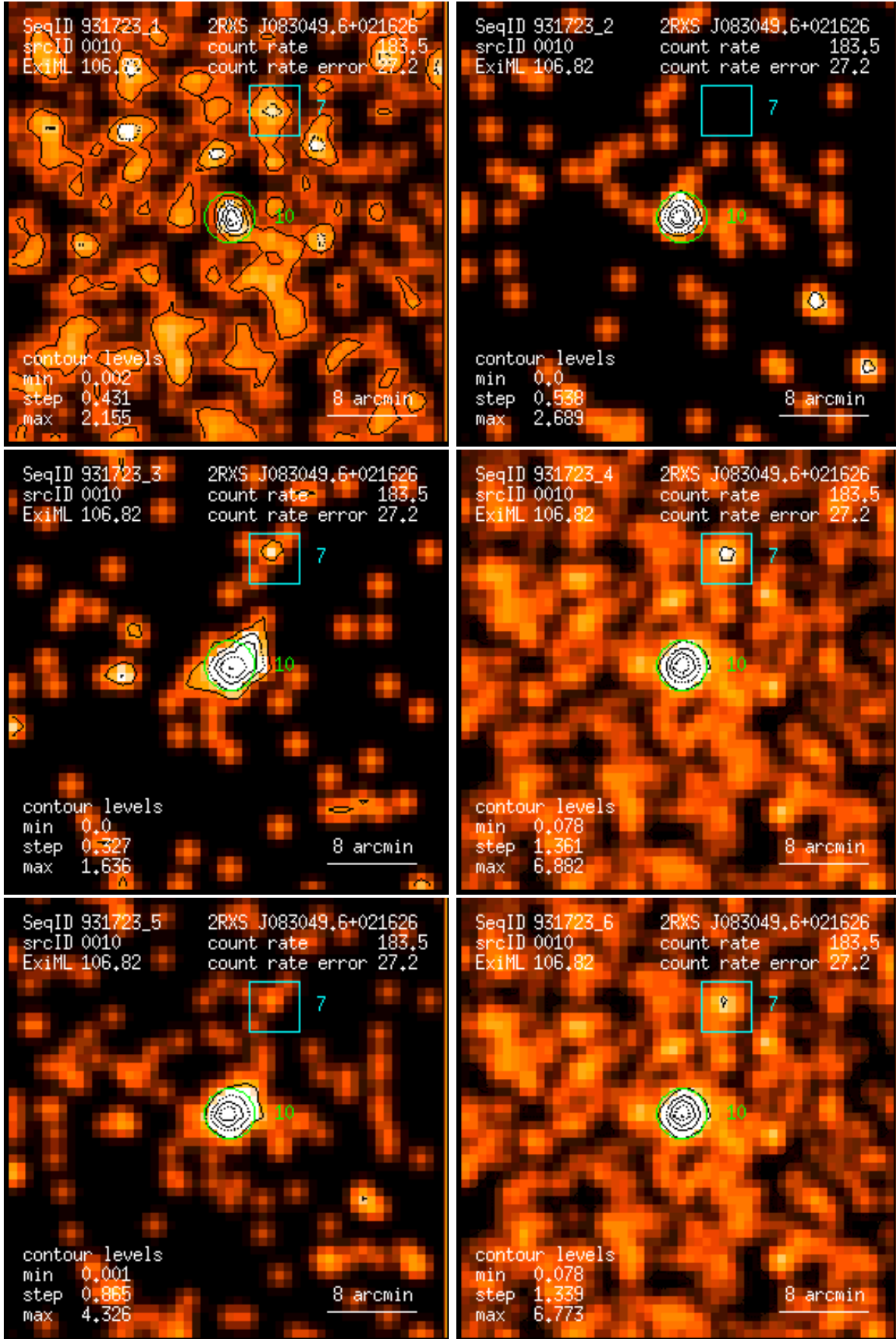
Figure 10: RASS 931723: detection 0010: band rate images, Gaussian filter: (1) PSPC channels 11 – 41, (2) 52 – 90, (3) 91 – 201, (4) 11 – 235, (5) 52 – 201, (6) 11 – 201. Broad band rates in counts/ks. Band rate contour levels in counts/ks/arcmin 2 .
