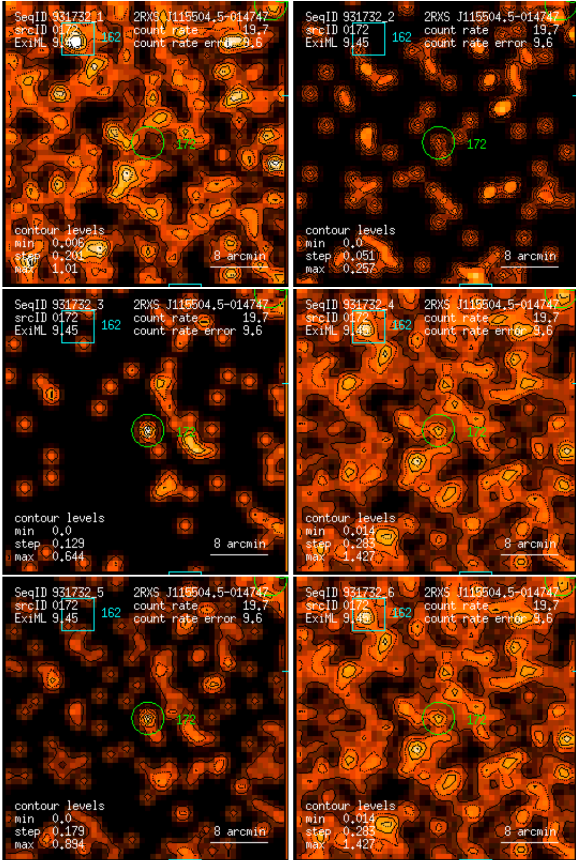
Figure 172: RASS 931732: detection 0172: band rate images, Gaussian filter: (1) PSPC channels 11 – 41, (2) 52 – 90, (3) 91 – 201, (4) 11 – 235, (5) 52 – 201, (6) 11 – 201. Broad band rates in counts/ks. Band rate contour levels in counts/ks/arcmin 2 .
