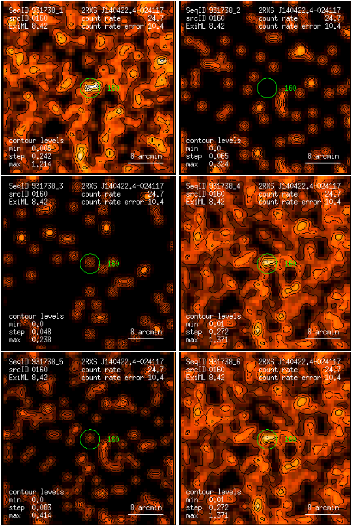
Figure 160: RASS 931738: detection 0160: band rate images, Gaussian filter: (1) PSPC channels 11 – 41, (2) 52 – 90, (3) 91 – 201, (4) 11 – 235, (5) 52 – 201, (6) 11 – 201. Broad band rates in counts/ks. Band rate contour levels in counts/ks/arcmin 2 .
