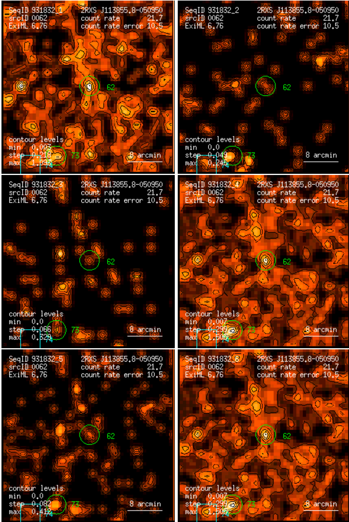
Figure 62: RASS 931832: detection 0062: band rate images, Gaussian filter: (1) PSPC channels 11 – 41, (2) 52 – 90, (3) 91 – 201, (4) 11 – 235, (5) 52 – 201, (6) 11 – 201. Broad band rates in counts/ks. Band rate contour levels in counts/ks/arcmin 2 .
