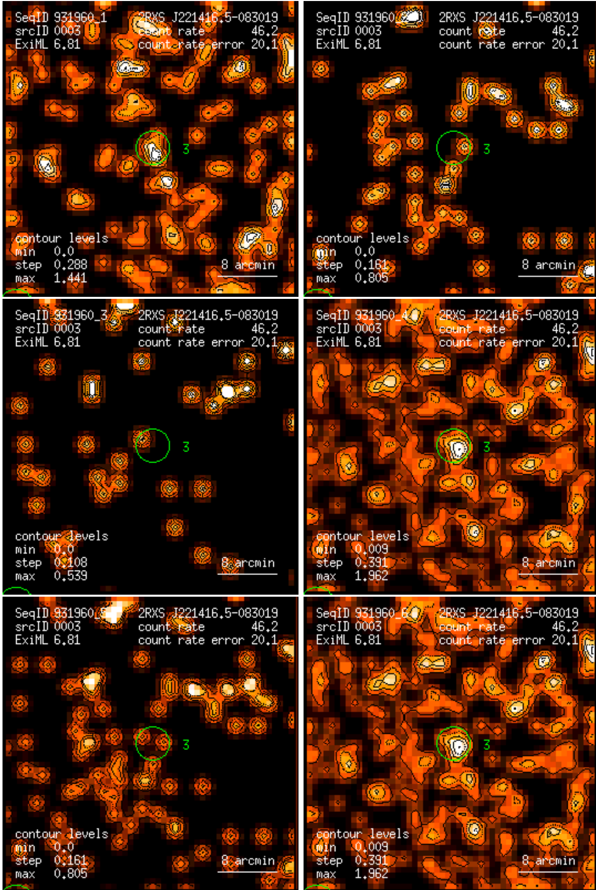
Figure 3: RASS 931960: detection 0003: band rate images, Gaussian filter: (1) PSC channels 11 – 41, (2) 52 – 90, (3) 91 – 201, (4) 11 – 235, (5) 52 – 201, (6) 11 – 201. Broad band rates in counts/ks. Band rate contour levels in counts/ks/arcmin 2 .
