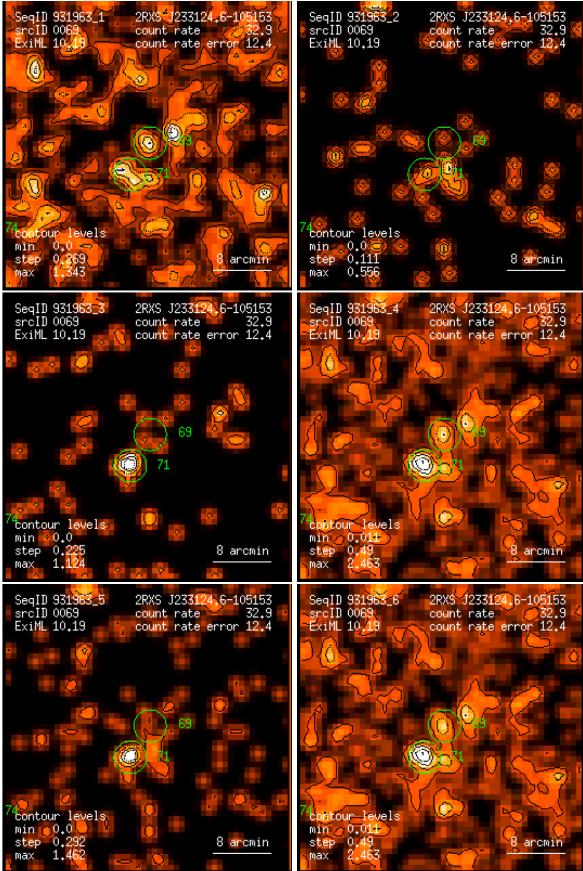
Figure 69: RASS 931963: detection 0069: band rate images, Gaussian filter: (1) PSPC channels 11 – 41, (2) 52 – 90, (3) 91 – 201, (4) 11 – 235, (5) 52 – 201, (6) 11 – 201. Broad band rates in counts/ks. Band rate contour levels in counts/ks/arcmin 2 .
