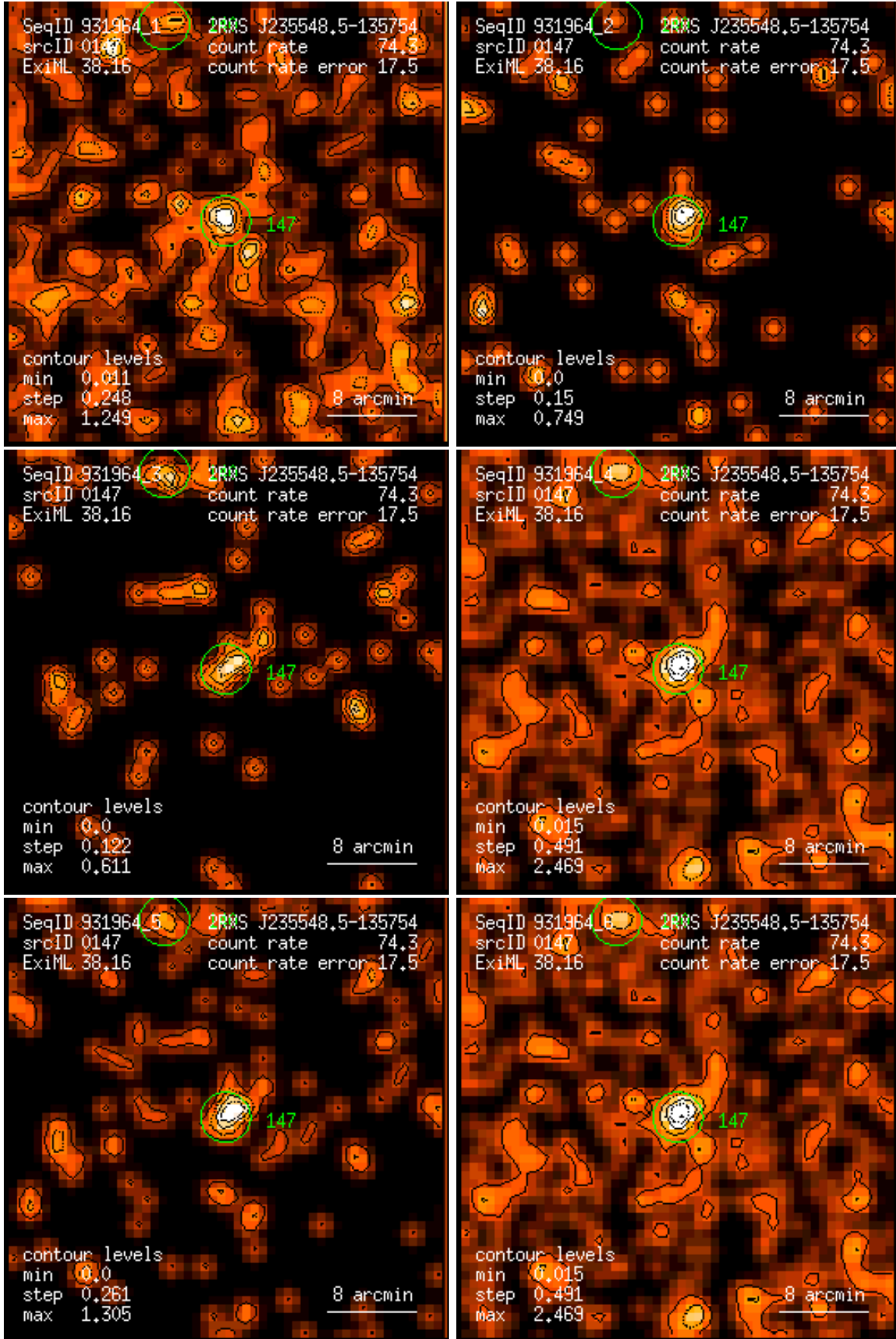
Figure 147: RASS 931964: detection 0147: band rate images, Gaussian filter: (1) PSPC channels 11 – 41, (2) 52 – 90, (3) 91 – 201, (4) 11 – 235, (5) 52 – 201, (6) 11 – 201. Broad band rates in counts/ks. Band rate contour levels in counts/ks/arcmin 2 .
