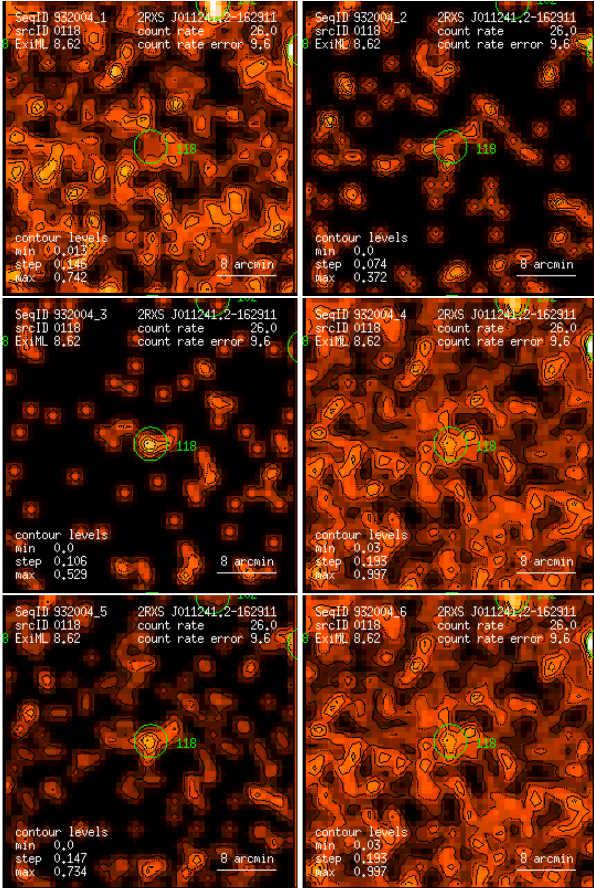
Figure 118: RASS 932004: detection 0118: band rate images, Gaussian filter: (1) PSPC channels 11 – 41, (2) 52 – 90, (3) 91 – 201, (4) 11 – 235, (5) 52 – 201, (6) 11 – 201. Broad band rates in counts/ks. Band rate contour levels in counts/ks/arcmin 2 .
