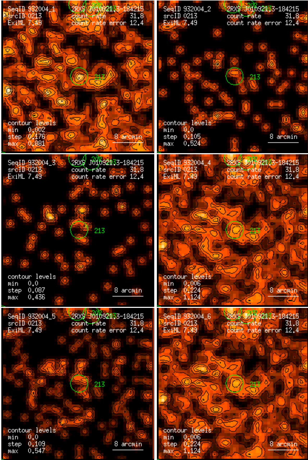
Figure 213: RASS 932004: detection 0213: band rate images, Gaussian filter: (1) PSPC channels 11 – 41, (2) 52 – 90, (3) 91 – 201, (4) 11 – 235, (5) 52 – 201, (6) 11 – 201. Broad band rates in counts/ks. Band rate contour levels in counts/ks/arcmin 2 .
