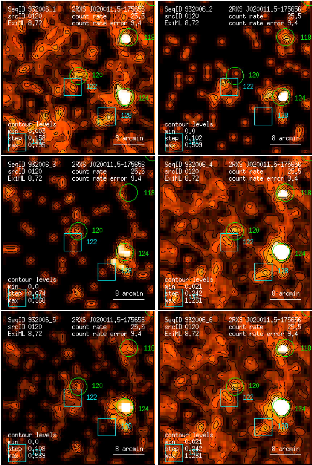
Figure 120: RASS 932006: detection 0120: band rate images, Gaussian filter: (1) PSPC channels 11 – 41, (2) 52 – 90, (3) 91 – 201, (4) 11 – 235, (5) 52 – 201, (6) 11 – 201. Broad band rates in counts/ks. Band rate contour levels in counts/ks/arcmin 2 .
