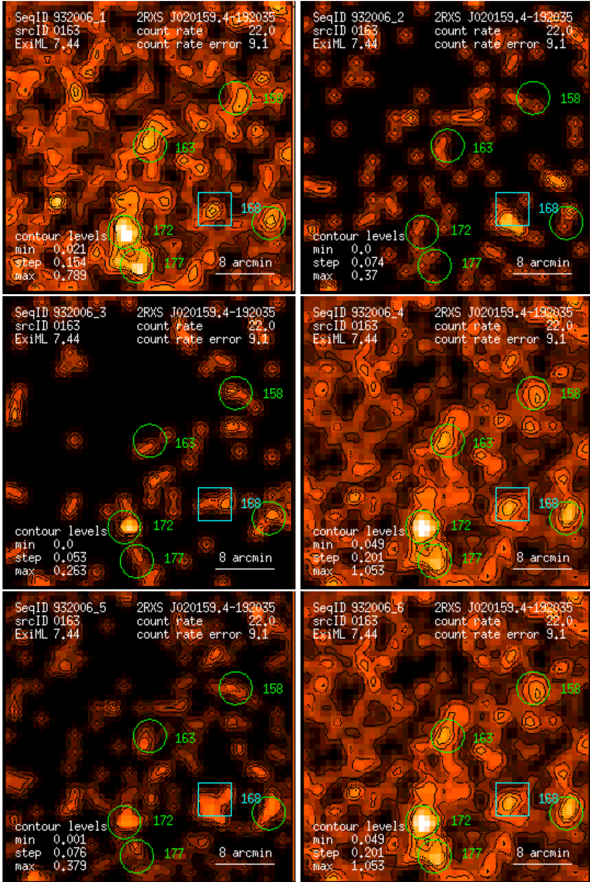
Figure 163: RASS 932006: detection 0163: band rate images, Gaussian filter: (1) PSPC channels 11 – 41, (2) 52 – 90, (3) 91 – 201, (4) 11 – 235, (5) 52 – 201, (6) 11 – 201. Broad band rates in counts/ks. Band rate contour levels in counts/ks/arcmin 2 .
