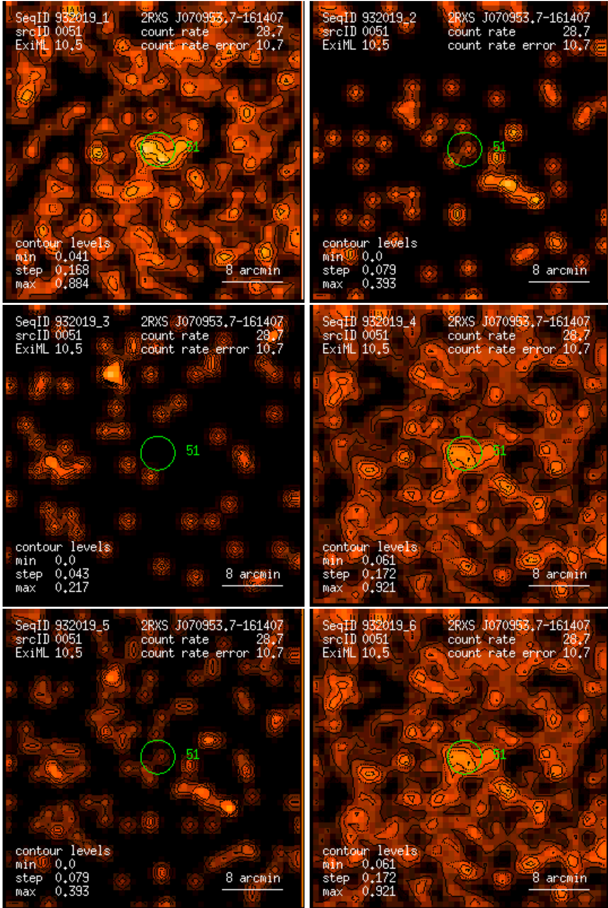
Figure 51: RASS 932019: detection 0051: band rate images, Gaussian filter: (1) PSC channels 11 – 41, (2) 52 – 90, (3) 91 – 201, (4) 11 – 235, (5) 52 – 201, (6) 11 – 201. Broad band rates in counts/ks. Band rate contour levels in counts/ks/arcmin 2 .
